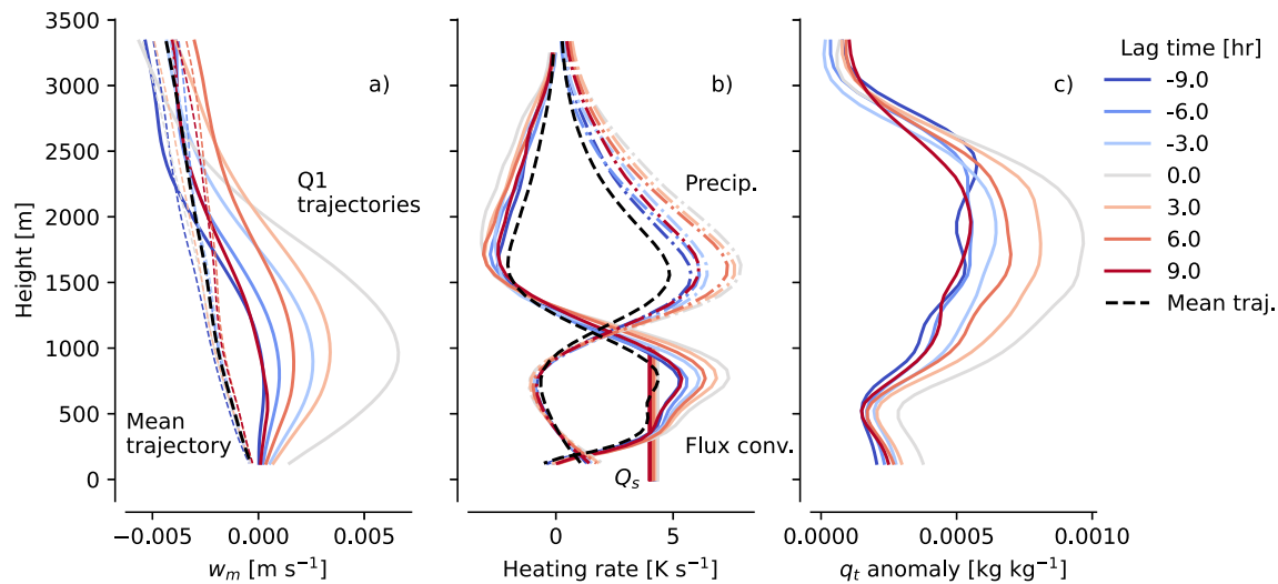
Figure 7. Profiles along Lagrangian trajectories characterizing the evolution in the quartile of 200 km blocks with the strongest D'_{sc_m} at zero lag, traced from 9 hr lead to 9 hr lag times along Lagrangian trajectories through the Icosahedral Nonhydrostatic Large-Eddy Simulation. (a) Vertical motion, where unbroken lines indicate trajectories along Q1 blocks, dotted lines indicate the evolution along the mean over all blocks, and black, broken lines represent the time-average over an average trajectory; (b) \theta'_{v,m} heating rates from Equation 8, decomposed into contributions from the convergence of (w'\theta'_v)_m (unbroken lines) and P_m (dash-dotted lines), and the evolution of the surface-controlled heating Q_s (vertical lines, Equation 12); (c) q_r anomaly in Q1 trajectories with respect to a mean trajectory. All profiles are averaged over the 79 launch times.
