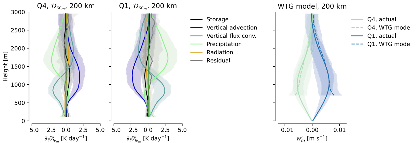
Figure 4. Left and central columns: Budgets of \theta'_{lv} averaged over the entire simulation period, in 200 km blocks, composited by D'_{sc_m} (Q4 and Q1), as in Figure 3. Right column: w'_m as diagnosed directly from the simulations (unbroken lines, “actual”), and from the Weak Temperature Gradient model for w'_m (Equation 8), plotted only above 700 m where gradients in \theta_v become appreciable. Shading captures the temporal interquartile range.
