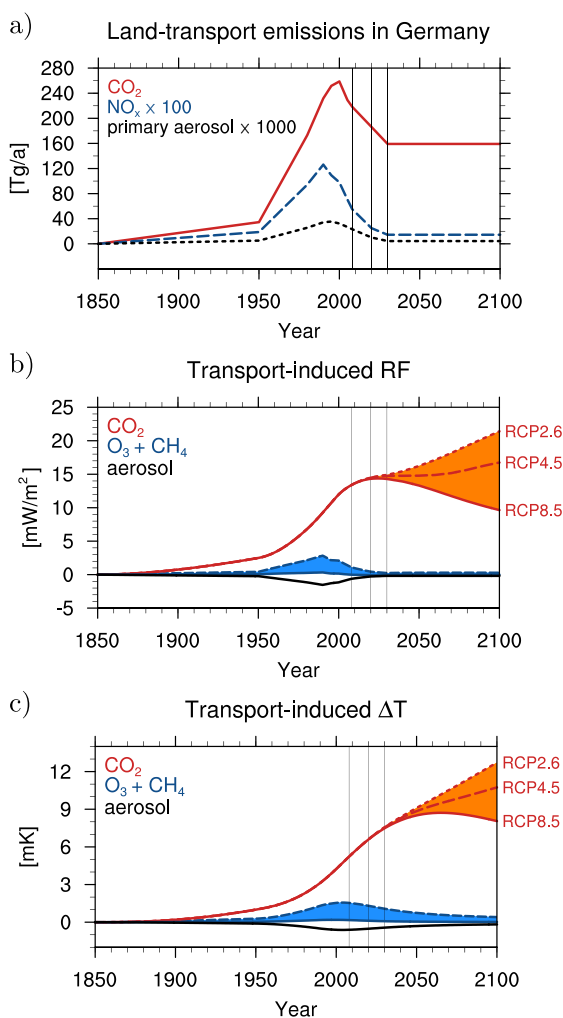
Fig. 7. Temporal change of (a) the transport-induced emissions of \text{CO}_2 , \text{NO}_x (expressed as \text{NO} equivalent, multiplied by 100), and particulate matter (primary aerosol, i.e., BC and POM, multiplied by 1000) assumed for Germany between 1850 and 2100 as well as (b) the resulting radiative forcings (RF) and (c) changes in global mean surface temperature ( \Delta T ) simulated with AirClim. The vertical lines indicate the years covered by the VEU emission data set. The different solutions for future radiative forcing and temperature change due to \text{CO}_2 result from different assumptions on future \text{CO}_2 background concentrations according to different future scenarios (RCP2.6, RCP4.5, and RCP8.5). Effects of \text{CH}_4 differ only slightly among the scenarios. Hence, \text{O}_3 + \text{CH}_4 values are shown for RCP8.5 only. The blue shaded area denotes the uncertainty ranging from \text{O}_3 + \text{CH}_4 to 5 \cdot \text{O}_3 + \text{CH}_4 . For values obtained for selected years in the different AirClim simulations, we refer to Table 3. Note that aerosol effects resulting from \text{SO}_2 emissions are not considered. See text for more details on this simplification.
