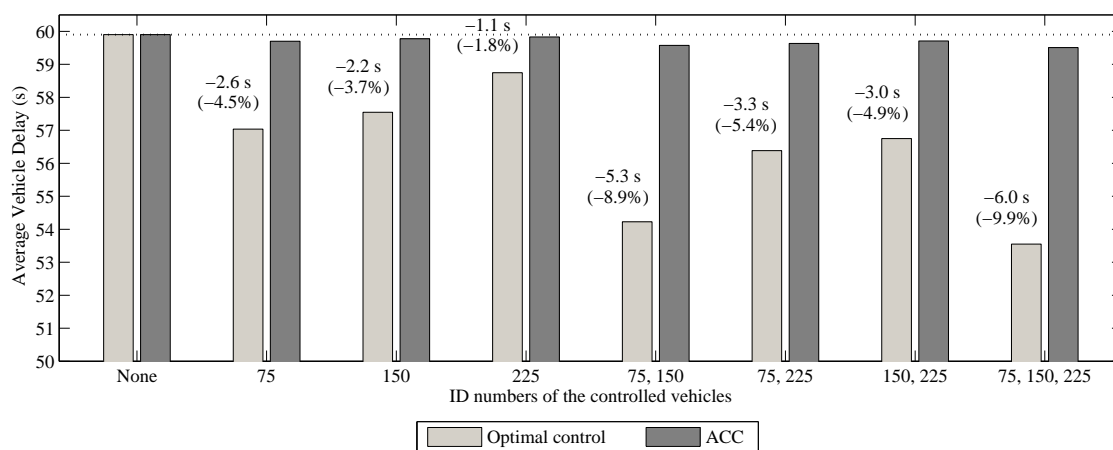
Figure 6: Average vehicle delay (AVD) in the no-control scenario, the optimal control scenarios and the ACC scenarios. The numbers on top of the light-gray bars indicate the difference in AVD and the difference in relative AVD reduction in comparison with the no-control scenario between the optimal control scenarios and the ACC scenarios with the same M .
