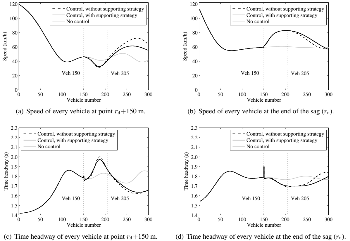
Figure 12: Speed and time headway of every vehicle on the first part of the sag and at the end of the sag in the no-control scenario, in the control scenario with M = \{150\} (optimal solution) and in the virtual scenario without supporting strategy corresponding to that control scenario.
