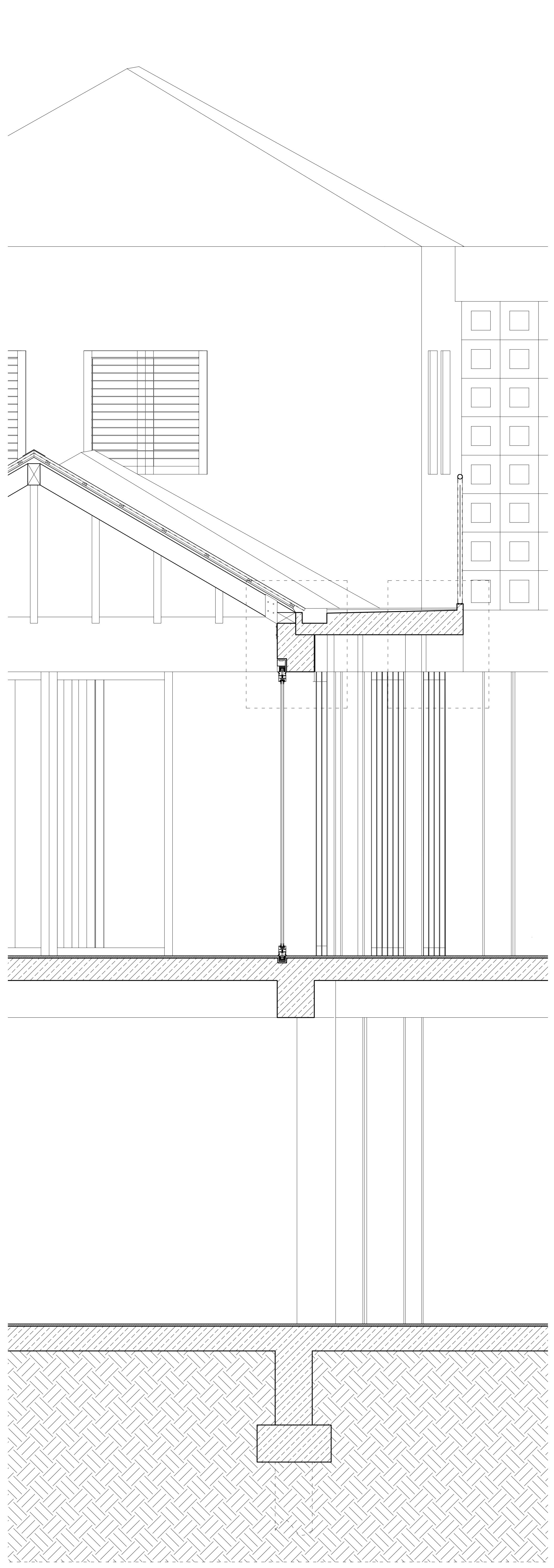
scale 1:20
