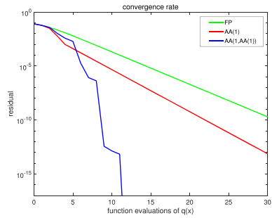
(b) x_0 = [0.2, 0.1]^T , convergence rate
