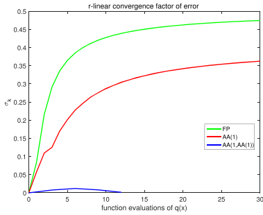
(a) x_0 = [0.2, 0.1]^T , convergence factor
