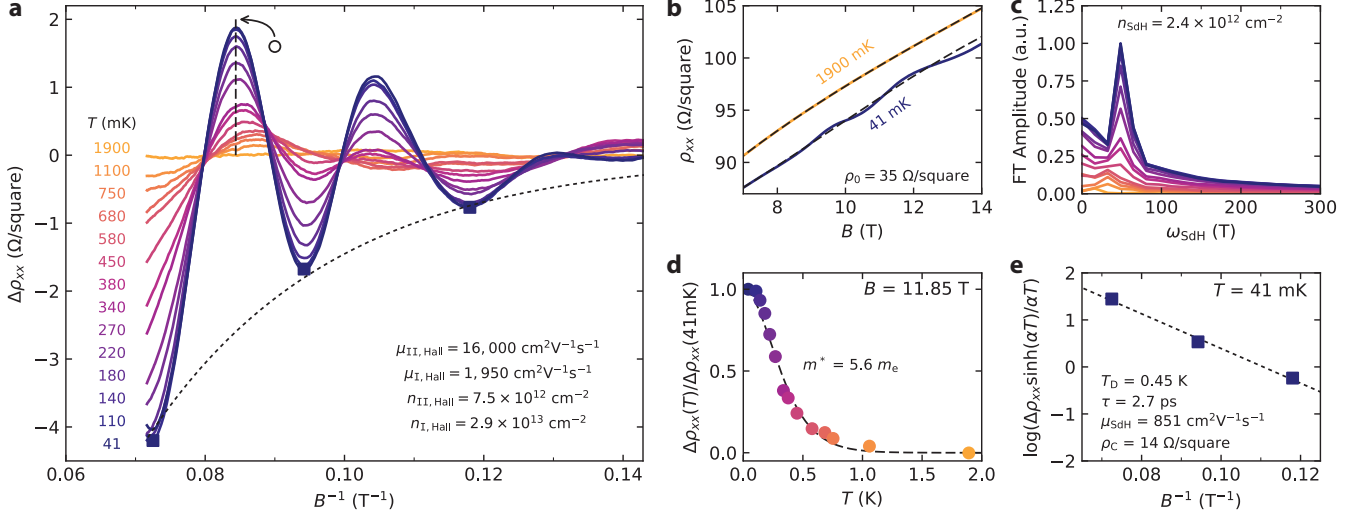
FIG. 5. Quantum oscillations of conductance. (a) Temperature dependence of the SdH oscillations after the removal of a 3 rd order polynomial background. The dashed and dotted lines indicate the data in (d) and (e), respectively. (b) Raw \rho_{xx} data at two different temperatures showing the fit of the polynomial background (dashed lines). (c) Fourier spectra of the oscillations in the range 7 T to 14 T. (d) Temperature dependence of the oscillations amplitude at B = 11.85 T and fit to eq. (2) (dashed line) from which the carrier effective mass m^* is extracted. (e) Dingle plot of the SdH oscillations minima at T = 41 mK and fit to eq. (2) (dotted line) from which the Dingle temperature T_D , elastic scattering time \tau , mobility \mu_{\text{SdH}} and the classical sheet resistance \rho_c are extracted.
