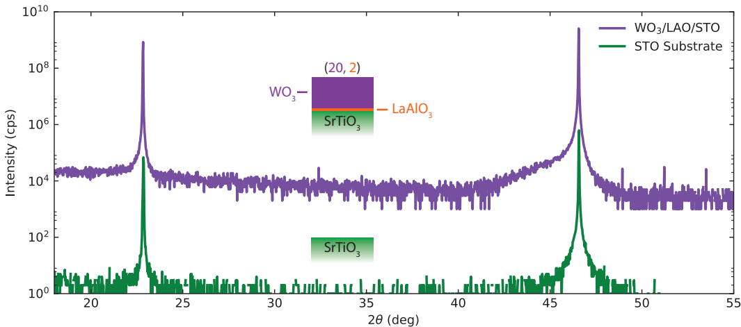
Supplementary Figure 2. XRD comparison of an STO substrate and a (20, 2) WO 3 /LAO/STO heterostructure. The \theta - 2\theta X-ray diffraction scan around the (001) and (002) substrate peak shows no clear diffraction peak coming from the heterostructure, further confirming the amorphous nature of our WO 3 overlayer.
