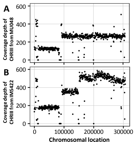
Figure 4: Depth of coverage analysis of Chromosome III (CHRIII) from unevolved strain IMU048 ( A ) and the evolved strain IMS422 ( B ). Sequencing reads from the IMU048 and IMS422 have been mapped onto the CEN.PK113-7D genome sequence (Nijkamp et al. 2012). Read count data represent the average coverage of non overlapping 500 bp window. These data are representative of the other two evolved strains (IMS423 and IMS424).
