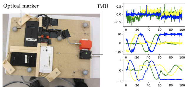
Fig. 6. Real dataset (adapted from Fig. 4.2 and 4.3 in [3]). Left: A snapshot of the platform for collecting real dataset Right: Measurements from an accelerometer ( y_{a,t} , top), a gyroscope ( y_{\omega,t} , middle) and a magnetometer ( y_{m,t} , bottom) for 100 seconds of data collected with the IMU showed in the left figure.).
