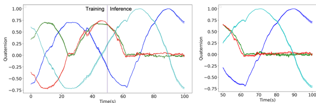
Fig. 7. Quaternion for real data. The solid, dotted and dashed lines correspond to ground truth, integrated and estimated quaternion respectively. The left and right figures are corresponding to scenarios 1 and 2 respectively. In the right figure, the dashed line is obtained by averaging over 50 independent trails.
