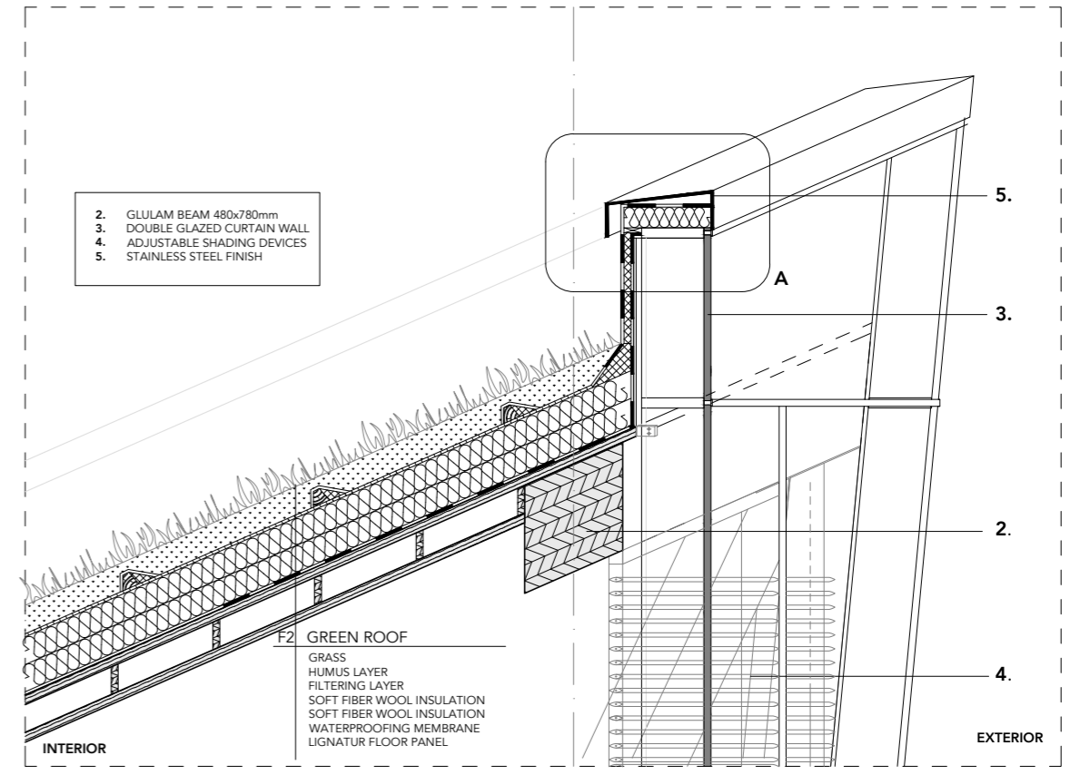
SECTION
