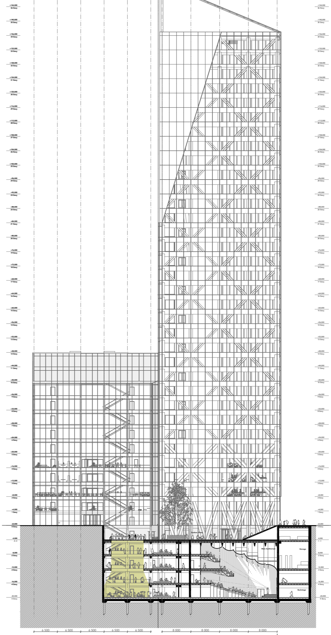
SECTION B
