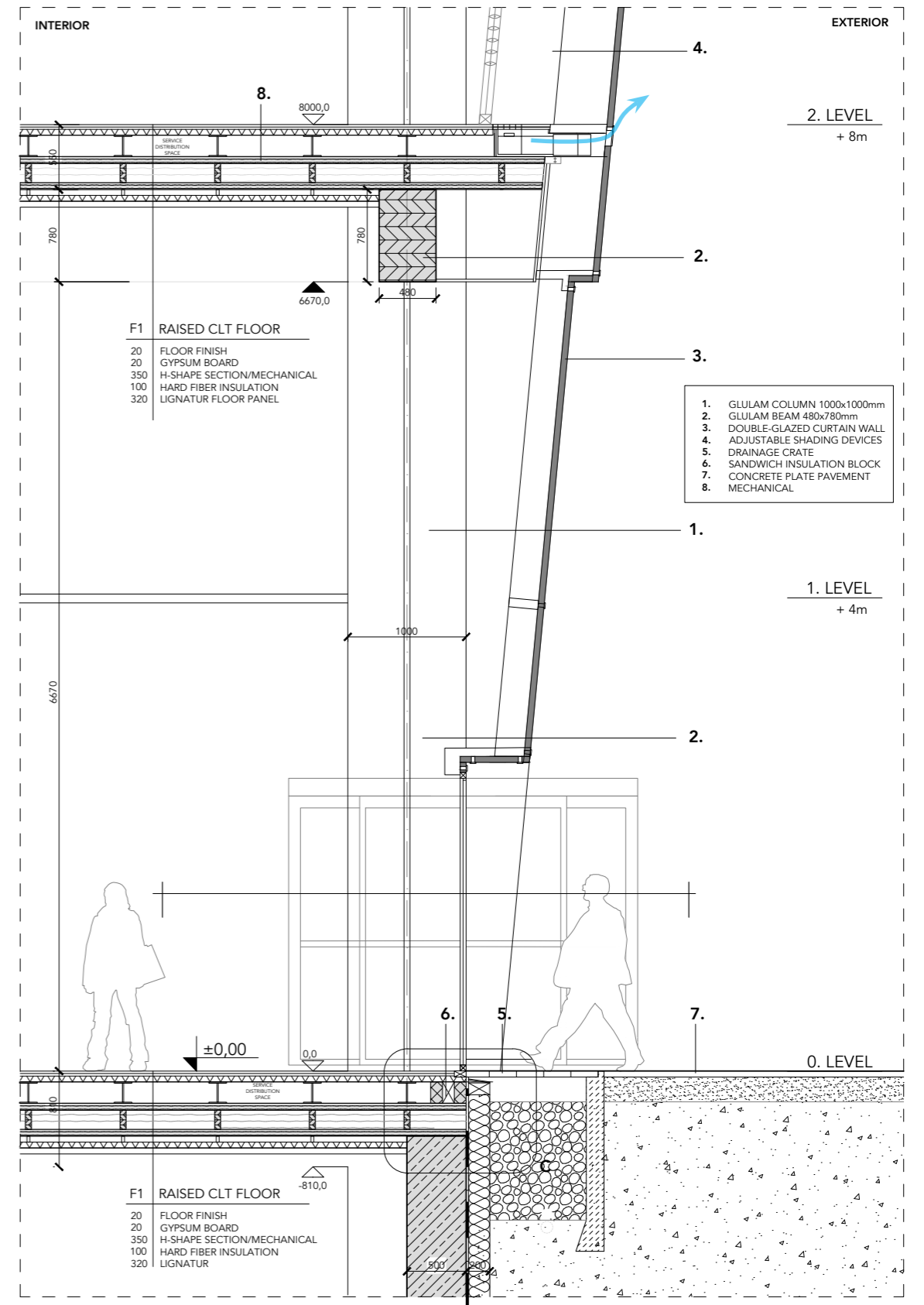
SECTION
