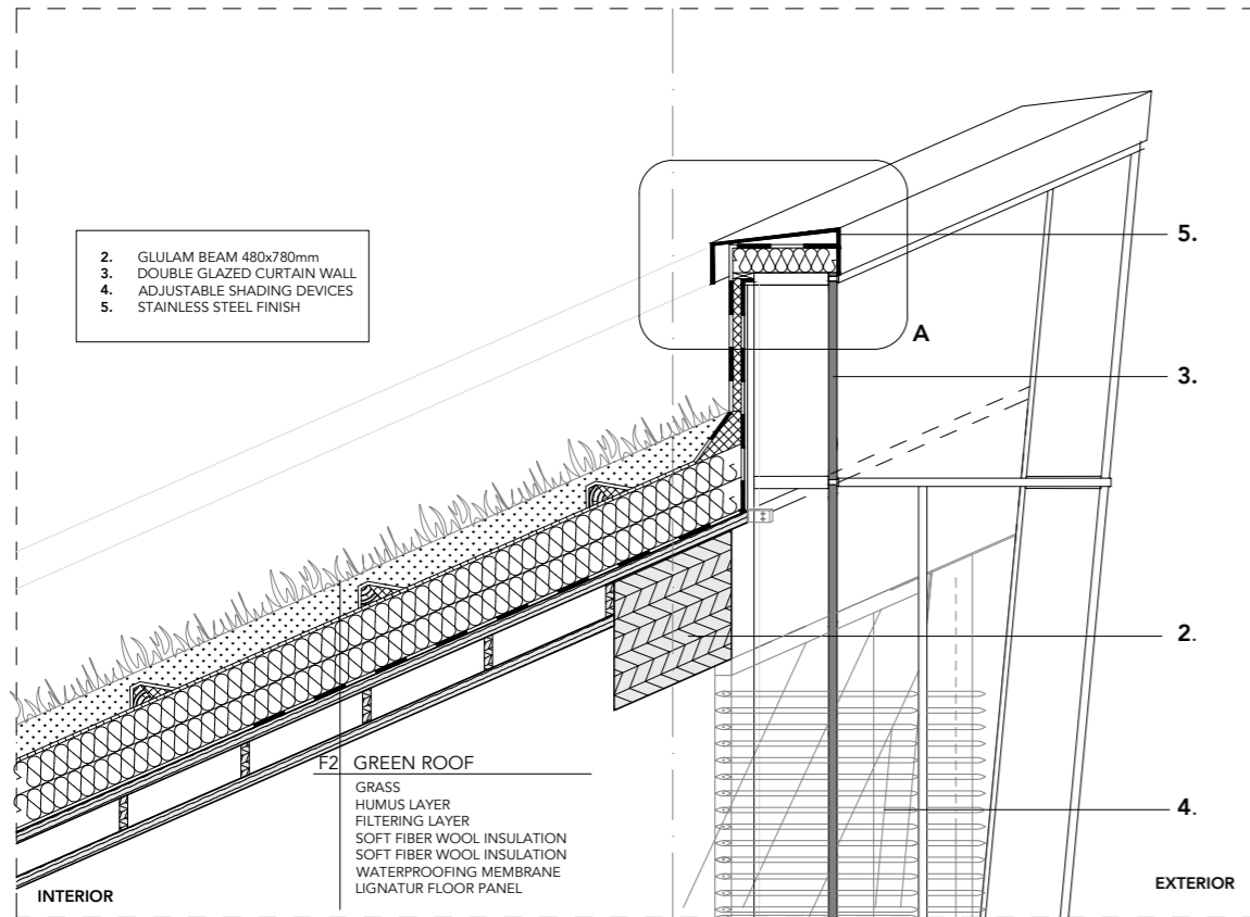
SECTION
