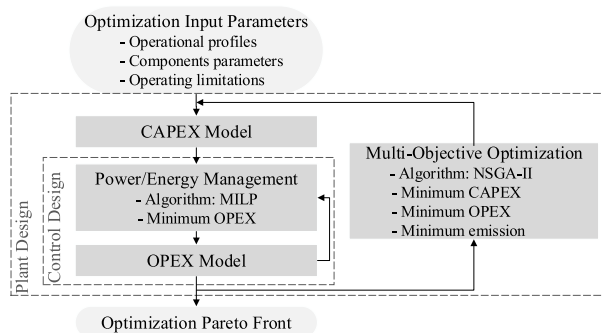
FIGURE 9. Optimization procedure.
