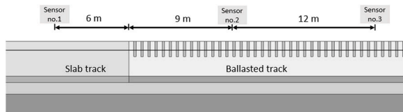
Fig. 5. Top view of transition model without auxiliary rail for validation.
