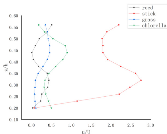
Fig. 3. Vertical distributions of point velocity for different types of vegetation of Q=20L/s , at the vertical 4
