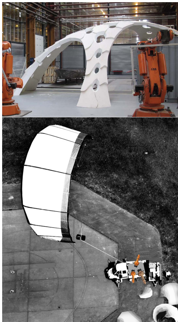
Figure 1. From laboratory to relevant environment - Impression of how D2RP could be moved from laboratory (top) to operation in situ and together with KP system (bottom) to produce affordable housing units
