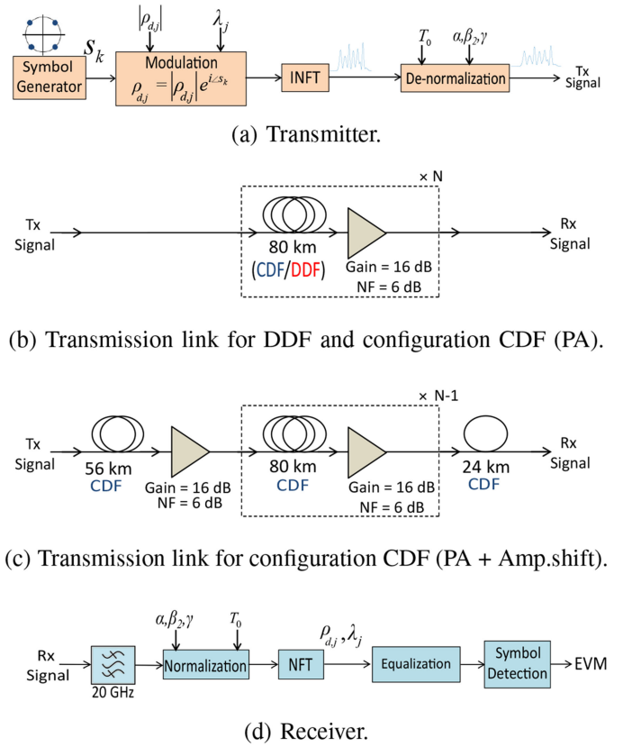
Fig. 2. Simulation setup of NFDN system with discrete spectrum modulation.
