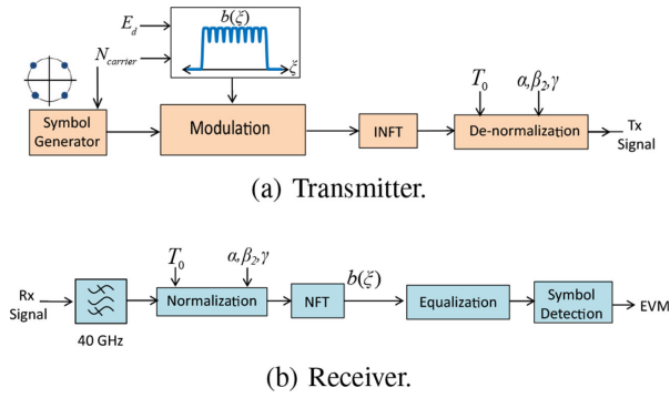
Fig. 7. Simulation setup of NFDN system with continuous spectrum modulation. The transmission link is the same as described before in Fig. 2(b), (c).
