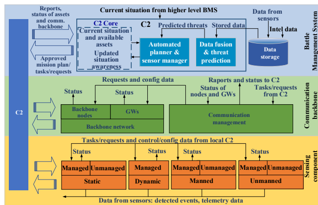
Fig. 4. Information flow.
