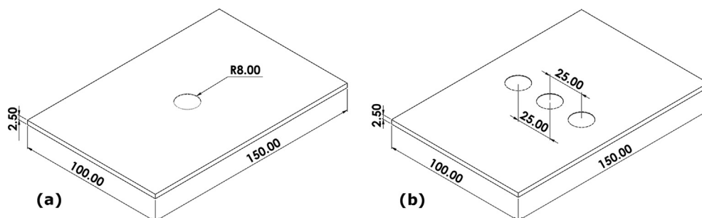
Fig. 2. Schematic of: (a) Single-impacted and (b) Multiple-impacted specimens (dimensions in mm).
