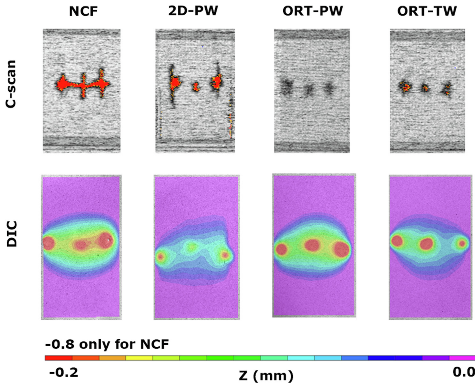
Fig. 5. C-scanning and DIC results for multiple-impacted specimens. (For interpretation of the references to colour in this figure legend, the reader is referred to the web version of this article.)
