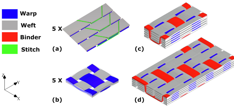
Fig. 1. Schematic of the different types of investigated composites: (a) NCF, (b) 2D-PW, (c) ORT-PW and (d) ORT-TW (The warp yarns highlighted in blue, the weft yarns in grey, the through thickness binders in red, and the stitch yarns for the non-crimp fabric (NCF) in green). (For interpretation of the references to colour in this figure legend, the reader is referred to the web version of this article.)
