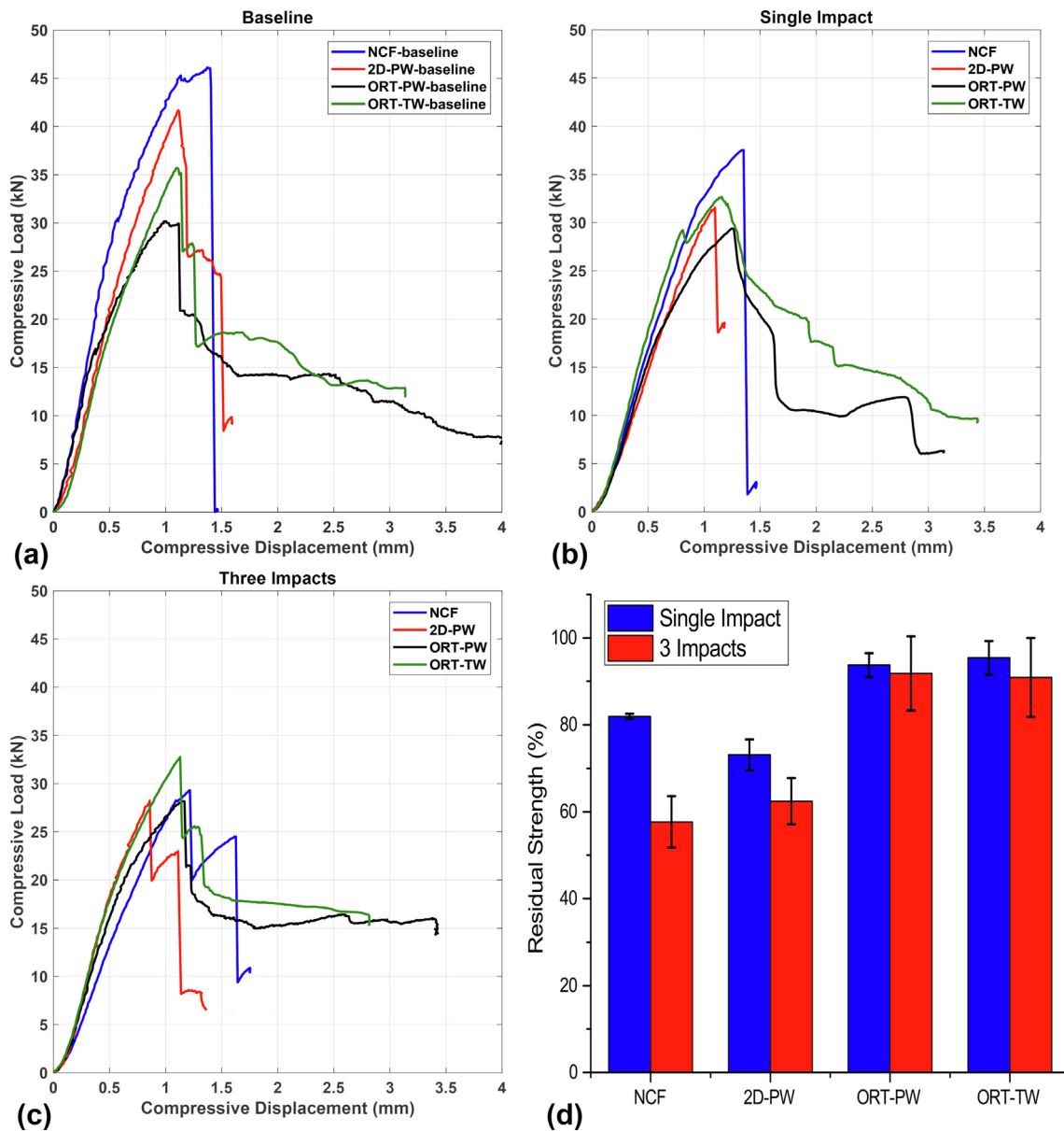
Fig. 10. Summary of the load-displacement curves for: (a) Baseline, (b) Single impact, (c) Multiple impact and (d) Residual strength for all the tested architectures. (For interpretation of the references to colour in this figure legend, the reader is referred to the web version of this article.)
