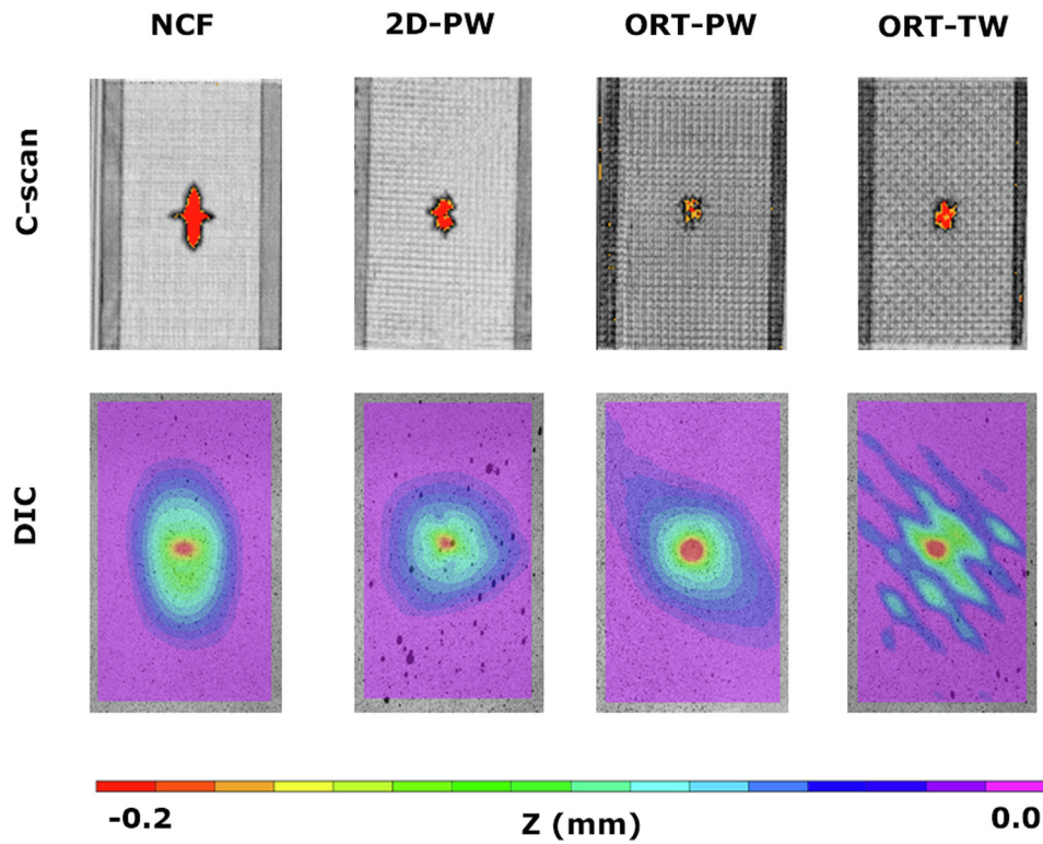
Fig. 4. C-scanning and DIC results for single-impacted specimens. (For interpretation of the references to colour in this figure legend, the reader is referred to the web version of this article.)
