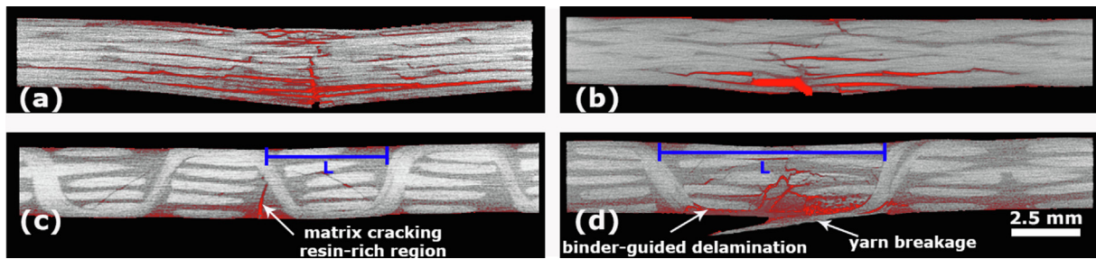
Fig. 8. X-ray CT cross-sections after impact for: (a) NCF, (b) 2D-PW, (c) ORT-PW and (d) ORT-TW. (For interpretation of the references to colour in this figure legend, the reader is referred to the web version of this article.)
