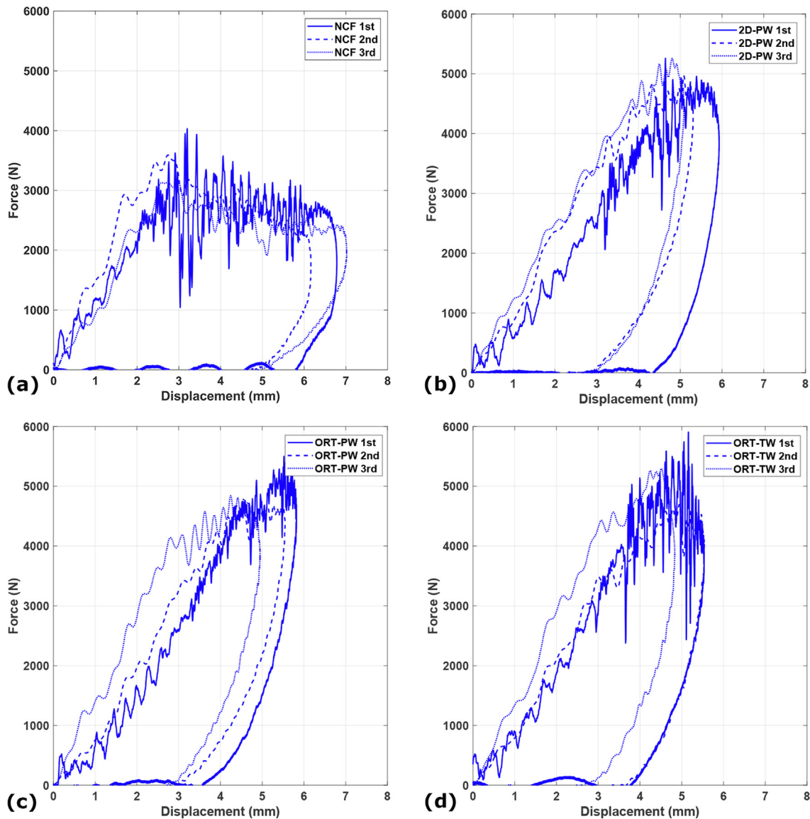
Fig. 6. Impact load-displacement curves for: (a) NCF, (b) 2D-PW, (c) ORT-PW and (d) ORT-TW. (For interpretation of the references to colour in this figure legend, the reader is referred to the web version of this article.)
