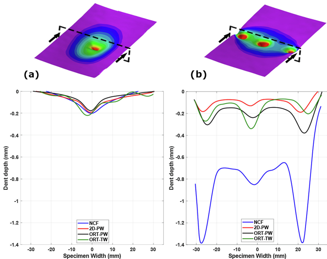
Fig. 9. Dent depth measured by the DIC: (a) Single and (b) Multiple impact. (For interpretation of the references to colour in this figure legend, the reader is referred to the web version of this article.)
