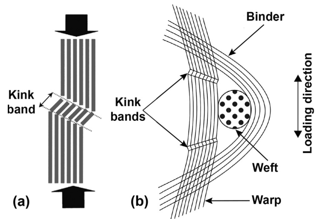
Fig. 11. Schematic of kink band formation: (a) 2D laminates, (b) 3D woven composites.
