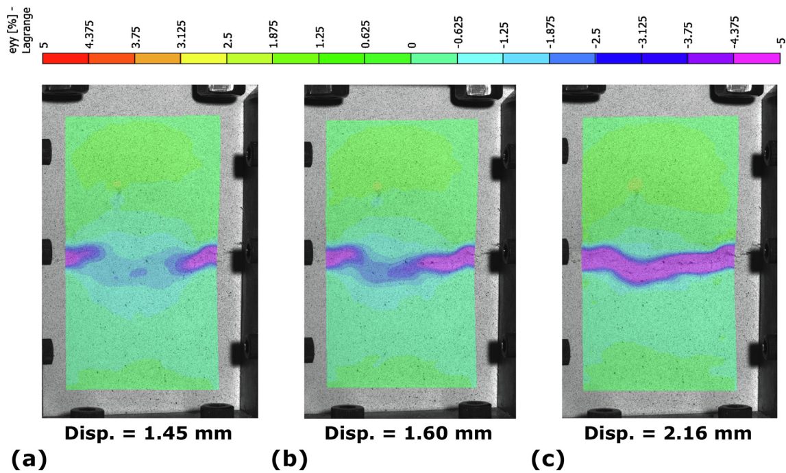
Fig. 13. Representative damage progression in CAI: (a) Side impacts damage, (b) Damage growth from the edges to the central impact; (c) Damage spans the full width of the specimen. (For interpretation of the references to colour in this figure legend, the reader is referred to the web version of this article.)
