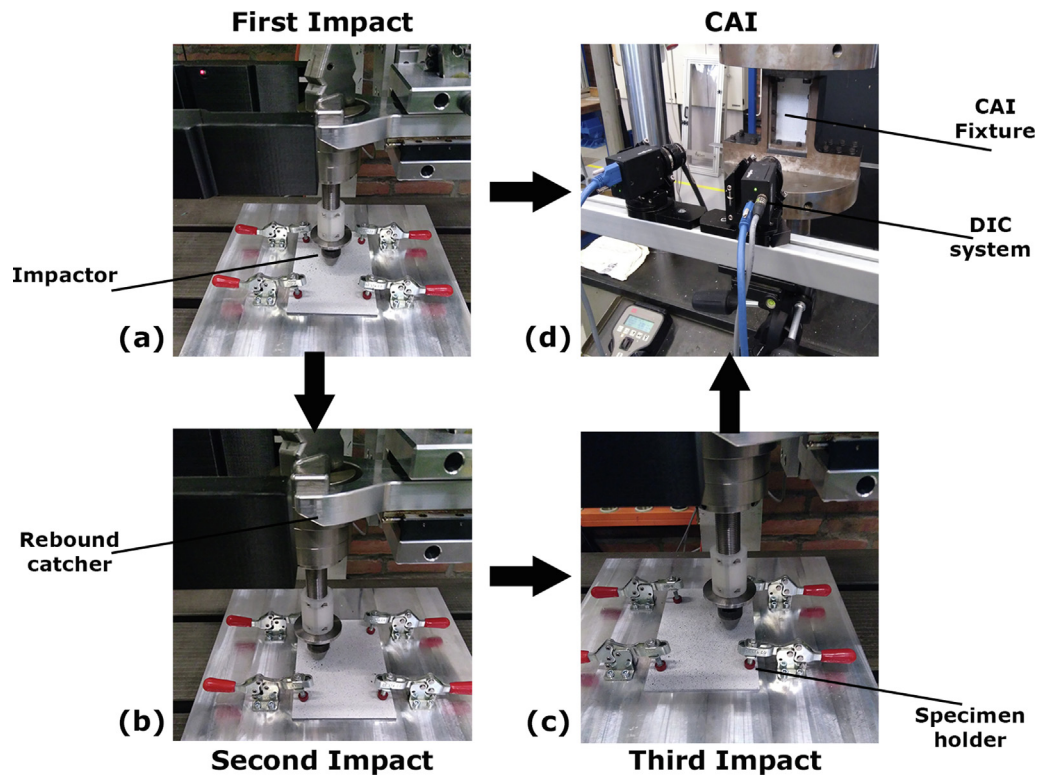
Fig. 3. Testing setup: (a) First impact, (b) Second impact, (c) Third impact and (d) CAI. (For interpretation of the references to colour in this figure legend, the reader is referred to the web version of this article.)
