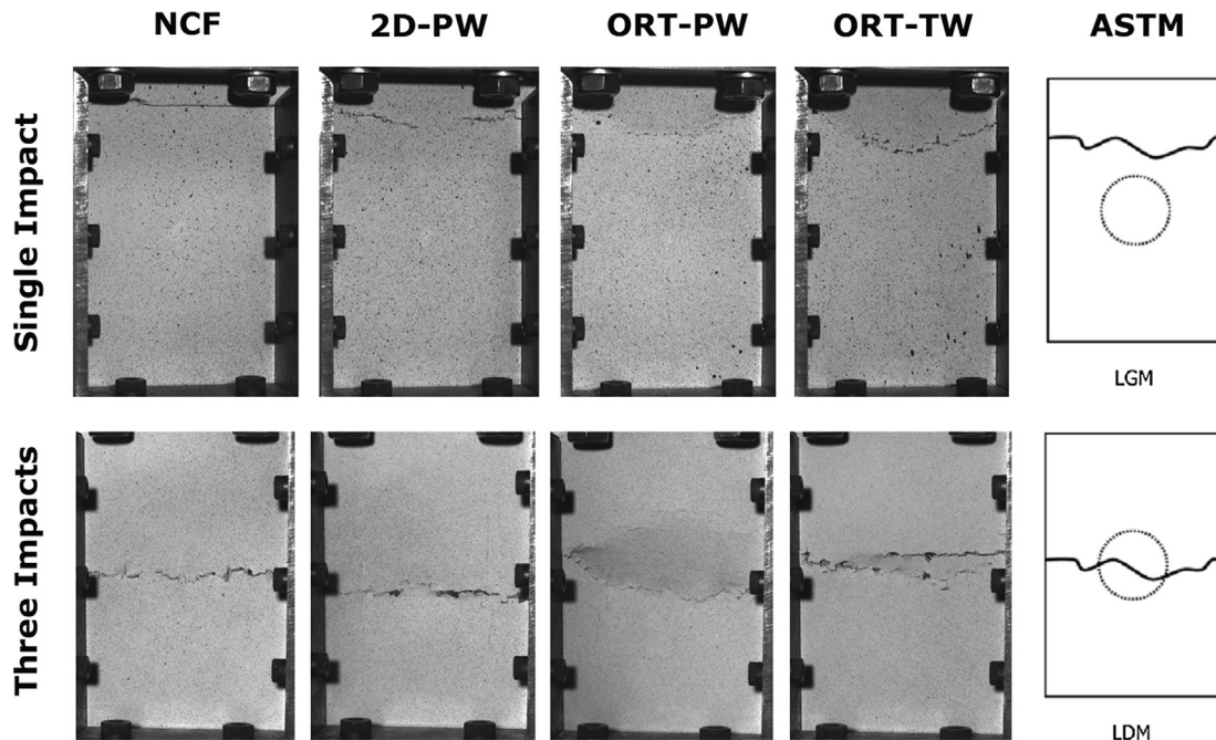
Fig. 12. Comparison of failure of: (a) Single impact and (b) Multiple impact specimens for all architectures.
