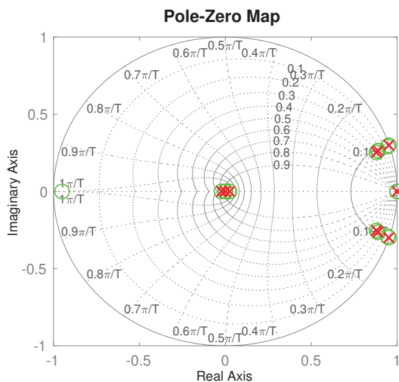
Fig. 8: Poles-zeros map with active damping
