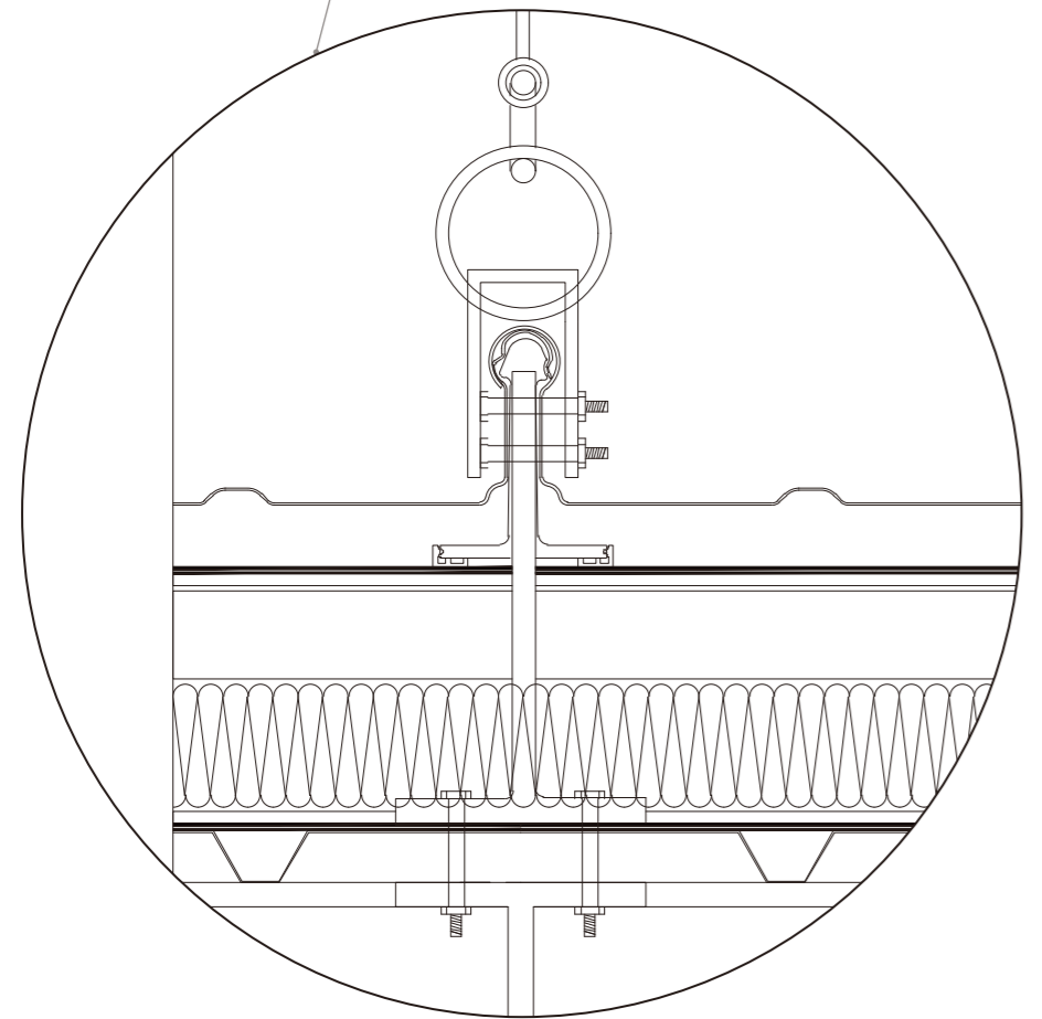
DETAIL A 1:10
