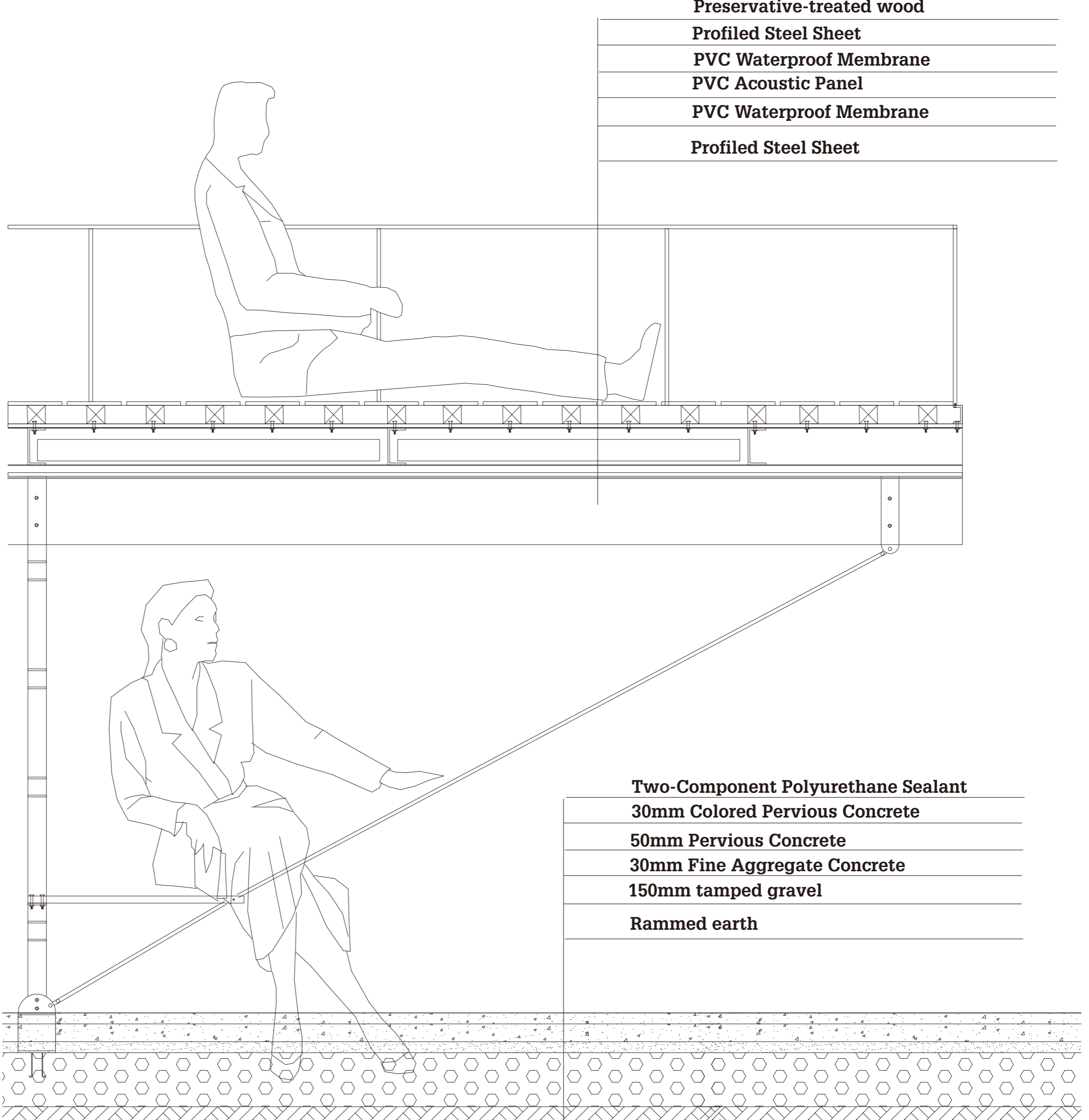
DETAIL B 1:10
