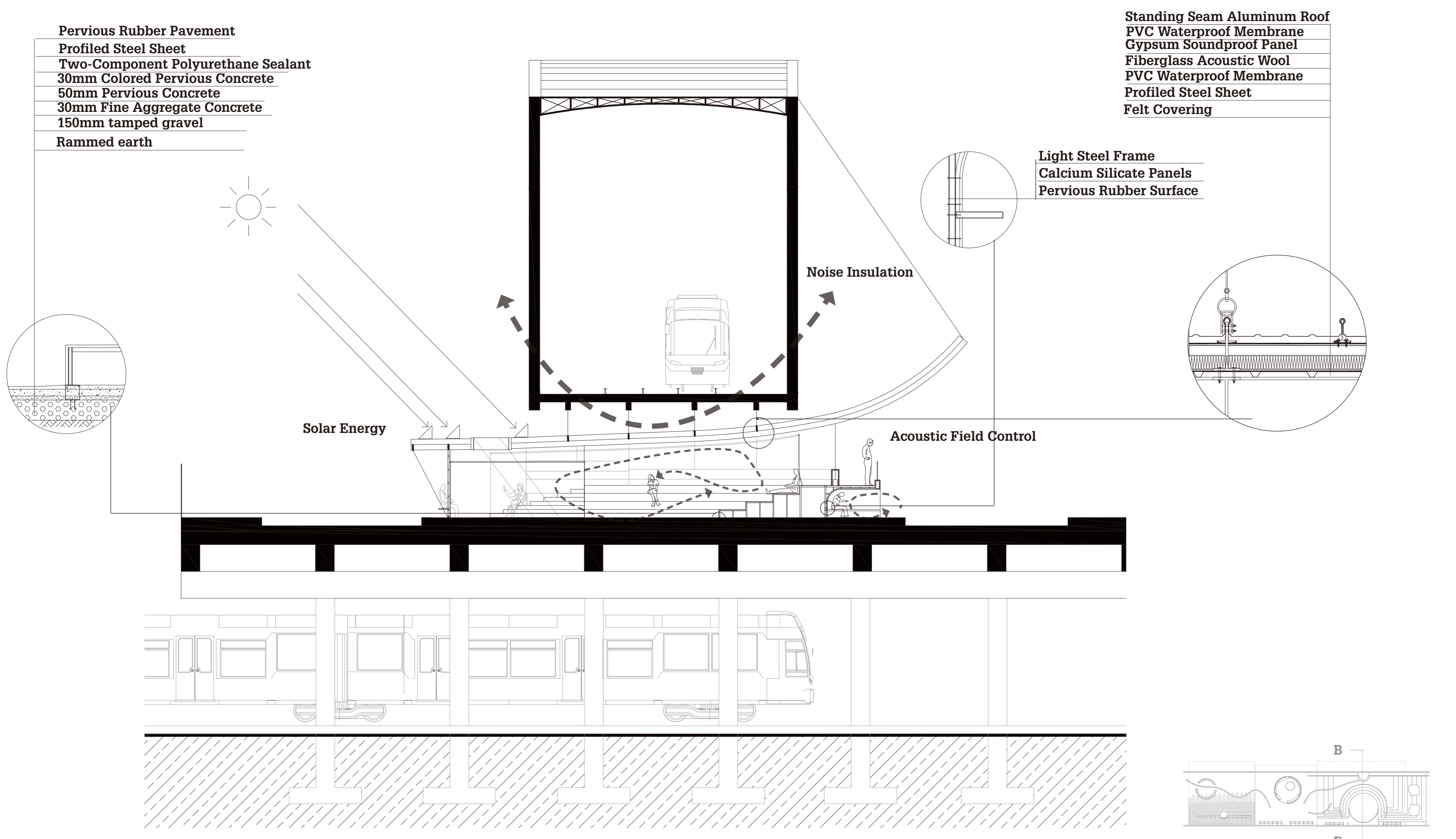
SECTION B-B 1:100
