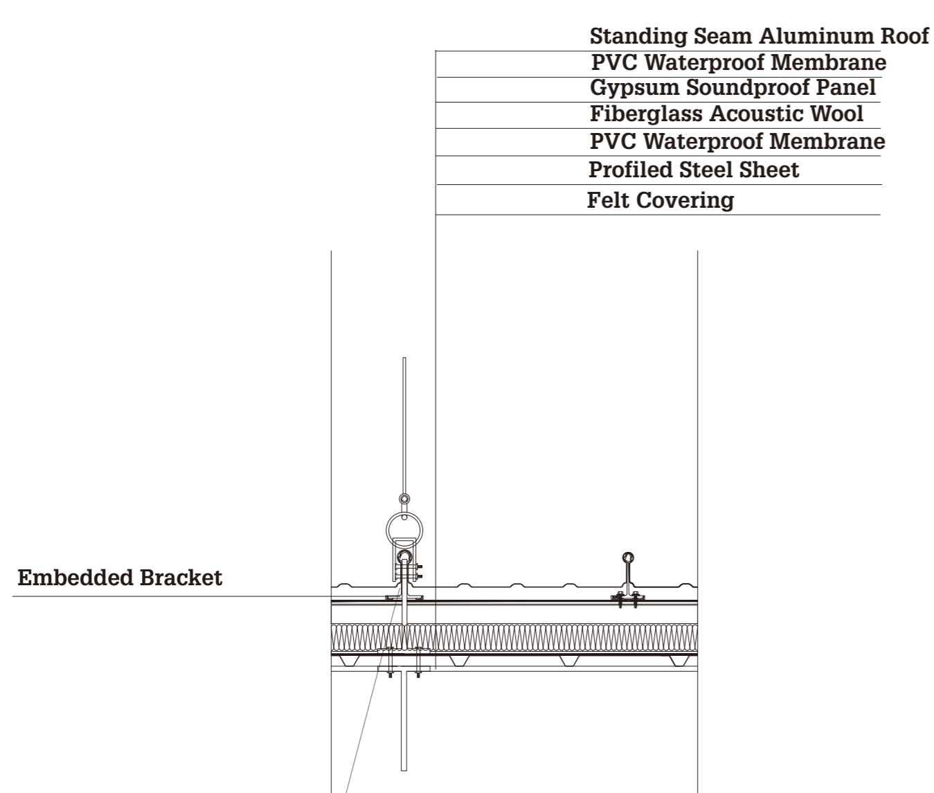
DETAIL A 1:10
