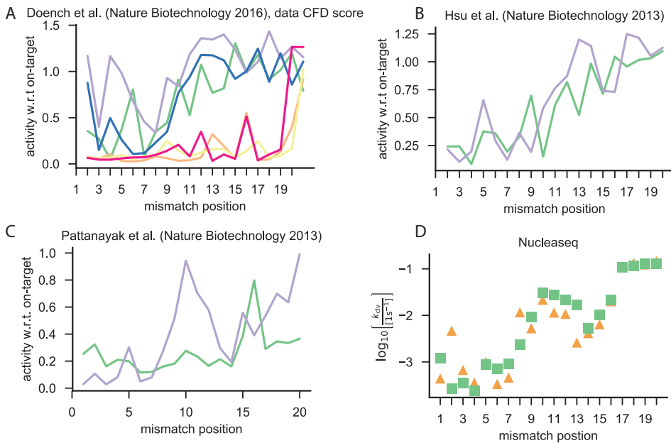
Figure S3.5: related to Figure ??, comparing single-mismatch profiles for various guides (data taken across the literature). (A) Cleavage activity w.r.t on-target, for different guides. Data from Doench et al. [?] (processed dataset from Zhang et al. [?]). (B) Cleavage activity w.r.t on-target, for different guides. Data from Hsu et al. [?] (processed dataset from Zhang et al. [?]). (C) Cleavage activity w.r.t on-target, for different guides. Data from Pattanayak et al. [?]. (D) NucleaSeq data for guide used throughout this study (orange triangles) and a second guide (green squares).
