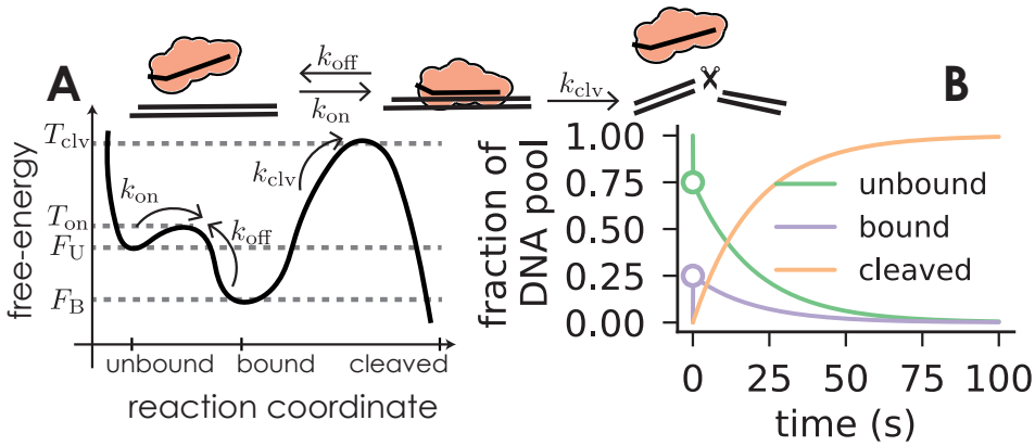
Figure 1.12: Same reaction as in Figure ??, but now with much higher rates of binding and unbinding. (A) Free-energy landscape. (B) Solution to Master equation tracks populations of all the three states over time. Dots indicate equilibrium fractions of bound/unbound DNA calculated using the Detailed balance condition of eq (??).
