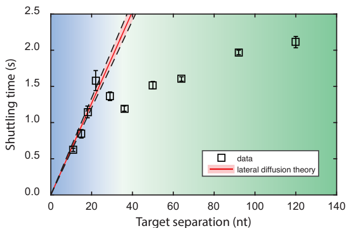
Figure 5.3: CbAgo shuttling behaviour differs across short and large distances Shuttling time is plotted versus distance between targets. Squares indicate the mean shuttling time for each DNA construct. The plotted error bars indicate the 95% confidence interval of 10^5 bootstrapped dwell times. The red line indicates the lateral diffusion model where the first four data points are fitted with k_{\text{esc}} = 15.8\text{s}^{-1} . The shaded red region indicates its 95% confidence interval. The blue region indicates where the shuttling time follows lateral diffusion theory. This theory breaks down for larger distances (green).
