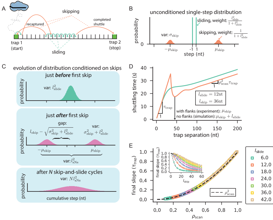
Figure 6.2: Modeling skip-and-slide search (shuttling events). (A) Schematic of shuttling event. Starting from the leftmost trap, the protein uses a combination of single-nucleotide steps (sliding) and larger steps (skipping) to reach the opposite trap after possibly getting recaptured at the initial traps several times. (B) single-step distribution of random walk defining our model. The protein either slides to a neighboring site or skips to sites located at \pm(\mu_{\text{skip}} \pm \sigma_{\text{skip}}) . (C) Distribution of visited sites conditioned on skips. (top) The protein covers a rms distance l_{\text{slide}}^2 between consecutive skips. (middle) The first skip takes the protein \mu_{\text{skip}} away (in either direction) with an uncertainty of \sigma_{\text{skip}} in the landing site. (bottom) Repeated skip-and-slide (sNs) cycles result in a distribution that resembles a simple random walk (top panel) with an adjusted effective step length of l_{\text{sNs}} . (D) Representative numerical solutions (S.I.) for shuttling time versus trapping distance. (E) Final slope versus scanning density. Inset shows equivalent versus skipping length (see S.I. for values in parameter sweep).
