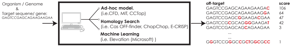
Figure 1.9: Existing predictions tools allow the user to provide the target gene locus & organism and output a ranked list of off-targets. Red nucleotides indicate mismatches.
