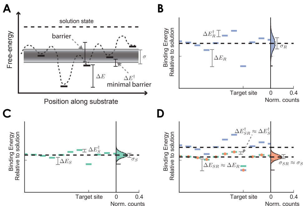
Figure 4.2: Search-stability paradox. (A) Energies of the binding sites are shown as short black horizontal markers. Being a sum of base pairing energies, binding energies are (approximately) Gaussian distributed with a standard deviation \sigma . The target site is separated from the other binding sites by an energy of about \Delta E . When diffusing laterally, the minimal barrier towards diffusion is set by the energetic difference between neighbouring sites ( \Delta E^\ddagger ). In reality there are intervening barriers, as depicted by the dashed line. With little loss of generality, we will ignore these additional contributions to the barriers and focus on the best-case scenario. (B) Recognition mode – Stable binding, but slow search: A larger difference between target and non-target energies comes at the cost of having larger barriers towards diffusion. The right panel shows the complete distribution of energetic states (standard deviation \sigma_R ) of which a subset is plotted in the left panel. The typical (minimal) barrier towards diffusion ( \Delta E_R^\ddagger ) and differential binding energy ( \Delta E_R ) are indicated. (C) Search mode – Fast search, but no stable binding: Decreasing the barriers also decreases the difference between target and non-target energy, which hampers the ability of the search complex to selectively bind to the target. The right panel shows the complete distribution of energetic states (standard deviation \sigma_S ) of which a subset is plotted in the left panel. The typical (minimal) barrier towards diffusion ( \Delta E_S^\ddagger ) and differential binding energy ( \Delta E_S ) are indicated. (D) Search + Recognition – Fast search and stable binding: If the search complex possesses (at least) two distinct binding modes, it becomes possible to combine the landscapes of figures B (blue) and C (green) to enable rapid diffusion ( \Delta E^\ddagger \approx \Delta E_S^\ddagger ) towards the target without loss of selectivity ( \Delta E \approx \Delta E_R ) (orange).
