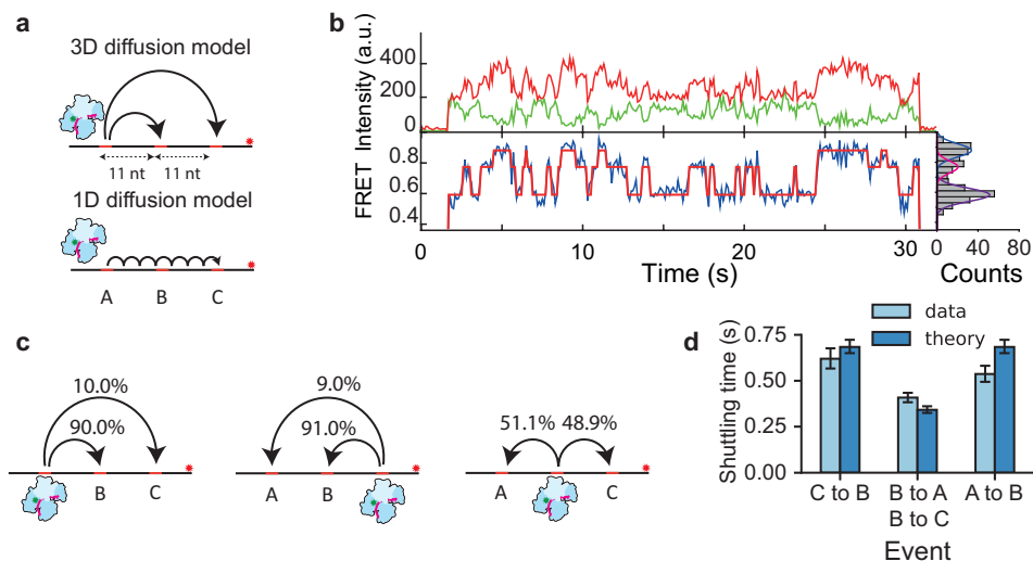
Figure 5.4: CbAgo undergoes short range diffusion through correlated steps. a, Models for target translocation at short range. In the 3D diffusion model, target dissociation occurs from A followed by random 3D diffusion through solution. In effect, the neighboring two targets (B and C) will compete for binding. In the lateral diffusion model, the CbAgo complex will have to bypass the adjacent target B before binding to target C. b, Representative FRET trace showing the shuttling behavior between three targets. Top: donor (green) and acceptor (red) intensities. Bottom: FRET trace (blue) and HMM assigned states (red). Right: The fitted states from this data trace with dark blue: state C, pink: state B and purple state A. c, Transition probabilities from state A to B,C (left), from state C to A and B (middle) and from state B to A or C (right). d, Experimental values of the shuttling time of the three target construct were compared against the parameter-free theoretical model that only uses the k_{\text{esc}} = 15.8\text{s}^{-1} from Figure 3. Error bars indicate the 95% confidence interval acquired from 10^5 bootstraps.
