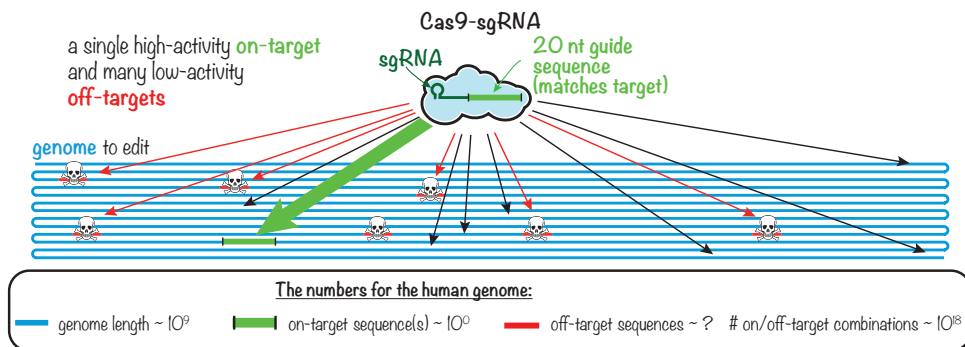
Figure 1.8: Although Cas9-sgRNA (or any other RGN of choice) predominantly targets the site that matches its guide (green), it is not perfect. The sheer volume of low frequency off-targeting events makes encountering an off-target more probable. Although not all off-target edits are necessarily harmful (red, as opposed to the black arrows), a single mistake can have consequences to the cell. Numbers in the inset are upper back-of-the-envelope estimates assuming a random genome of human length, and are meant to demonstrate the imbalance between on-target and the vast number of off-targets.
