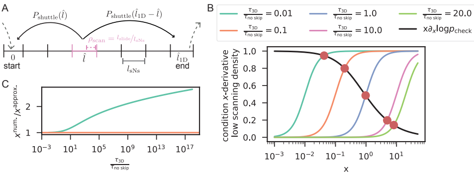
Figure S6.4: related to Figure ?? .derivation of search time at given scanning density. (A) Illustration of paths (and corresponding probabilities) that lead the protein from segment 1 to l_{1D} (size l_{sNs} ) without having interrogated all binding sites within segment l . Relates to Equation ?? . (B) At low scanning densities, the search time exhibits a unique minimum. Colored lines show right hand side of Equation ?? for varying values of \tau_{3D}/\tau_{\text{slow}} and black line shows the left hand side. Intersections (red dots) our found numerically and –together with Equation ?? -indicate the location in \{x, y\} -space the skip-and-slide optimum can be found at (Equation ??) . (C) Approximate location of skip-and-slide optimum ( x -coordinate) from Equation ?? versus numerical solution to Equation ?? .
