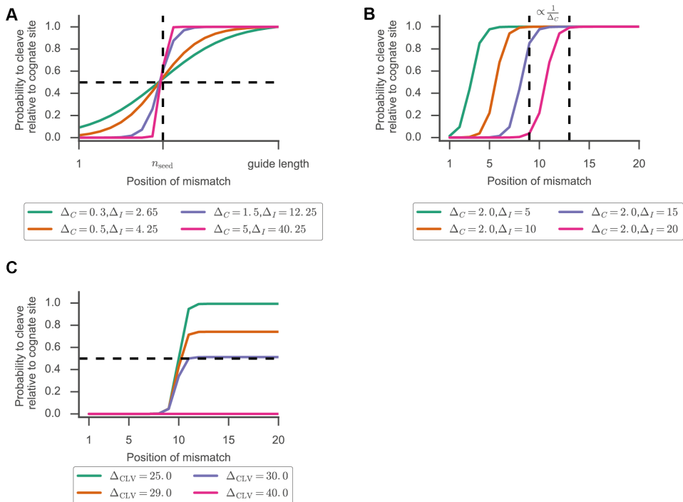
Figure S2.2: Single mismatch off-targets, related to figure ??. (A) Relative probability of cleaving a singly mismatched target. Seed length ( n_{seed} ) is kept constant by tuning \Delta_C and \Delta_I , while ensuring equation 2 of the main text is satisfied ( \Delta_{clv} = -100k_B T, \Delta_{PAM} = 0.25k_B T ). (B) The width of the transition region from seed to non-seed is set by the positive bias for correct base pairs ( \Delta_C ) ( \Delta_{clv} = -100k_B T, \Delta_{PAM} = 0.25k_B T ). (C) Tuning the intrinsic bias against cleavage ( \Delta_{clv} ) allows for differential targeting of sequences with PAM distal mismatches by shifting p_{max} of equation 1 of the main text ( \Delta_C = 3k_B T, \Delta_{PAM} = 3k_B T, \Delta_I = 30k_B T ).
