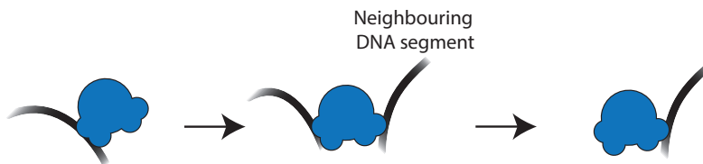
Figure S5.7: Cartoon representation of target search mechanisms. Sliding: Proteins that undergo sliding make a well-correlated movement along the contour of the nucleic acid substrate. There is no net displacement of counterions (grey circles). Hopping: Proteins alternate quickly between a bound and unbound state with respect to DNA and there is counterion condensation upon dissociation of the protein. The method of diffusion is similar to 3D search, but its movements are correlated along the contour of the strand. Intersegmental transfer: This mechanism is a specialized form of hopping where segments appear transiently close by allow the protein to transfer to this new segment.
