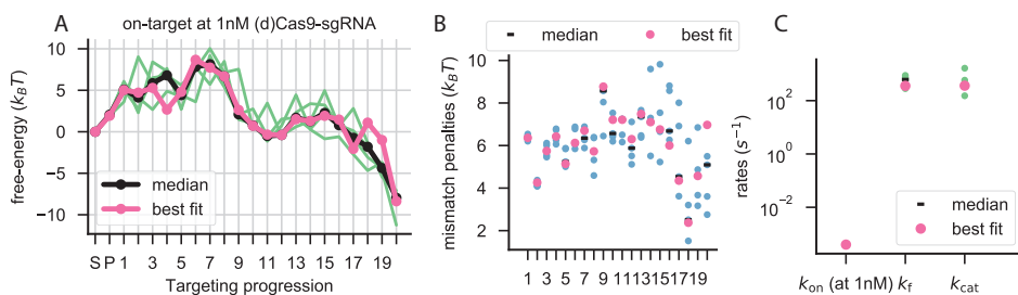
Figure S3.2: related to Figures ?? and ?. Simultaneous fit to HiTS-FLIP and NucleaSeq data. (A) Free-energy landscape for 1nM sgCas9-RNA interaction with on-target DNA. Green curves represent fit results from individual runs of our Simulated Annealing optimization algorithm whose resulting values differ less than 5% from the best-solution's outcomes (Figures ??A-B) (see S.I.). Black shows median to guide the eye. Pink shows best solution, used to produce Figures ??A-C. (B) Mismatch penalties as a function of position along the RNA-DNA hybrid. Blue dots show individual fit results (after selection). Black shows median to guide the eye. Pink shows best solution, used to produce Figures ??A-C. (C) Forward rate parameters. Green dots show individual fit results (after selection). Black shows median to guide the eye. Pink shows best solution, used to produce ??A-C.
