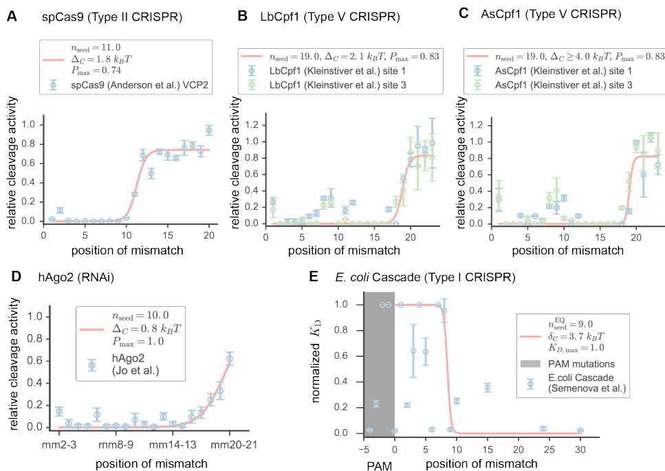
Figure 2.6: Comparison to experimental data. Fit of sigmoid (equation ??) to experimental data from: (A) spCas9 [? ]. (B) LbCpf1 [? ]. (C) AsCpf1 [? ]. (D) Human Argonaute 2 [? ]. (E) E. coli Cascade complex [? ]. Values reported in (A)-(D) correspond to the median of 1000 bootstrap replicates, and the confidence intervals in the text correspond to 68%. See Figure ?? for additional fits.
