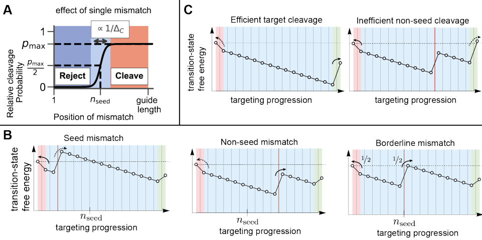
Figure 2.2: Rule (i) – seed region. (A) The relative-to-wildtype cleavage probability of a target with a single mismatch. Our model predicts a sigmoidal curve, with maximum off-target activity p_{\max} , seed length n_{\text{seed}} , and width of the seed to non-seed transition \sim 1/\Delta_C . See figure ?? for parametric sweeps. (B) Transition landscapes illustrating that the placement of a single mismatch (fltr: before, exactly at, beyond the seed’s border) influences the cleavage probability. (C) Increasing the kinetic bias against cleavage can suppress cleavage of off-targets with a PAM distal mismatch (compare right panel to right panel in (B)), while still maintaining a high on-target activity (left panel).
