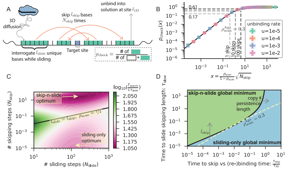
Figure 6.3: Optimal search times. (A) Schematic single search round. In search of the unique target, the protein uses a combination of skipping and sliding along the substrate before it unbinds into solution and must perform 3D diffusion before it can return. Only sites slid past (at least once) are interrogated (green), resulting in a probability p_{\text{check}} to interrogate a particular site. (B) Comparison of p_{\text{check}}(x) (solid line, Equation 3) to Monte Carlo simulations (symbols) (details given in Methods). Dashed lines indicate Argonautes ( \rho_{\text{scan}} \approx 0.3 ) that typically skip once (light grey), 10 (dark grey), and 100 times (black) before unbinding. (C) Search time versus N_{\text{slide}} and N_{\text{skip}} . Region above the solid line represents sparse scanning ( \rho_{\text{scan}} < 0.5 ), while the region below it represents dense scanning ( \rho_{\text{scan}} > 0.5 ). (D) Phase diagram showing when T_{\text{search}}^{\text{Ns}} < T_{\text{search}}^{\text{sliding}} . Dashed line represents the constant scanning density of 0.3 (approx. the value estimated for both Ago). Arrows represent directions of increasing l_{\text{skip}} , protein copy number (concentration) and substrate persistence length.
