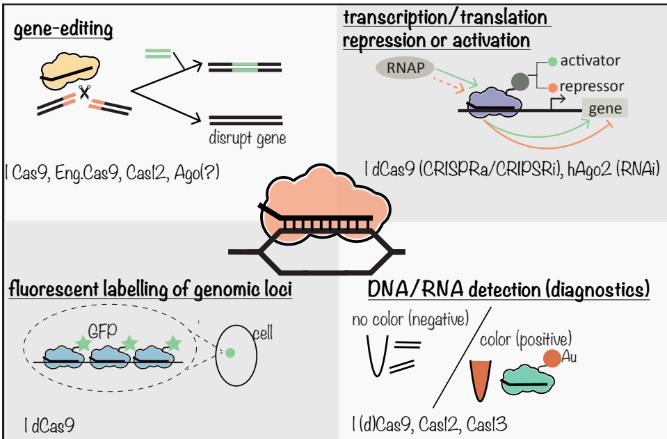
Figure 1.7: The “genome-engineering toolbox”. CRISPR-Cas9, CRISPR-Cas12, CRISPR-Cas13, and even Argonaute are utilized in many different ways (see text). From the perspective of our model, the different systems are fairly similar: a protein loaded with a guide that targets the complementary sequence.
