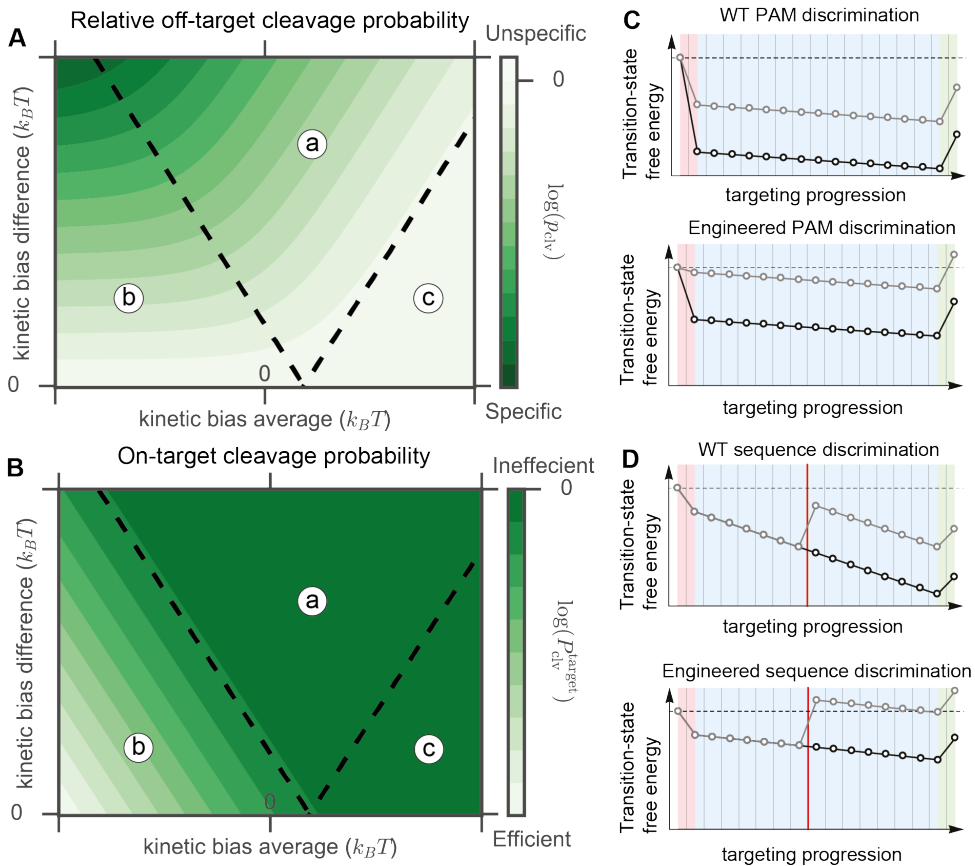
Figure 2.5: Rule (iv) – specificity-efficiency decoupling. (A) The cleavage probability on a fully cognate target but with a mismatched PAM, compared to one with the correct PAM, as a function of the average and difference in the kinetic bias of the correct and incorrect PAM. Independent of the sequence following both PAMs, one can identify three regimes (Supplemental Information). Only in regime a is the RGN's specificity improved through a decrease in the average PAM bias toward R-loop initiation. (B) On-target efficiency for the target with the correct PAM. In regime a, the RGN's efficiency is not compromised, allowing for simultaneous maintenance of on-target efficiency and specificity. (C) The cognate protospacer flanked by either a canonical PAM (black) or incorrect PAM (grey) is bound by a WT (top panel) or engineered RGN (panel). (D) A matched/mismatched protospacer (black/grey) bound by wildtype/engineered RGN (top/bottom panel).
