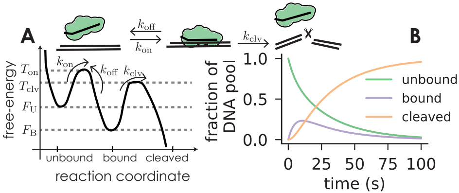
Figure 1.11: The RGN binds its substrate at a rate k_{on} . Before cleaving with rate k_{clv} , the RGN can unbind at a rate k_{off} . (A) Free-energy landscape. Stable states (minima) are denoted by F 's, while transition states between two configurations are indicated by T 's. (B) Solution to Master equation tracks populations of all the three states over time.
