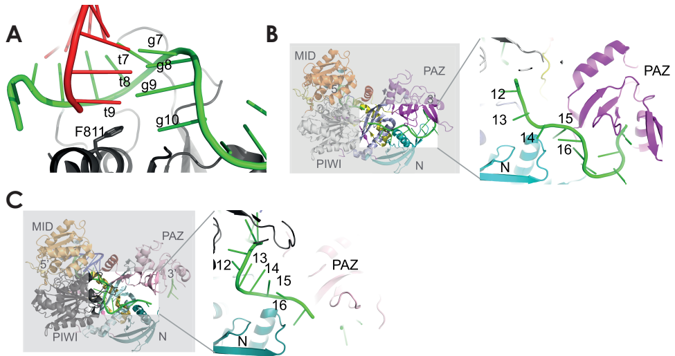
Figure 4.5: Cleavage competent state. (A) Structure showing the base pairing between a guide strand (green) and a target strand (red). The base pairing beyond nt 8(g8) is blocked by a residue F811 in a helix of the PIWI domain (snapshot of the structure 4W50 taken in pymol). (B) A binary structure of hAgo2-miRNA showing the disordered 3' supplementary region of guide RNA (green) passing through a channel between N domain (blue) and PAZ domain (purple) (snapshot of the structure 4W5N taken in pymol). (C) A ternary structure of hAgo2-miRNA and its target showing an A-form helical arrangement of the 3' supplementary region of guide (green) in ternary structure (snapshot of the structure 4W50 taken in pymol). sites
