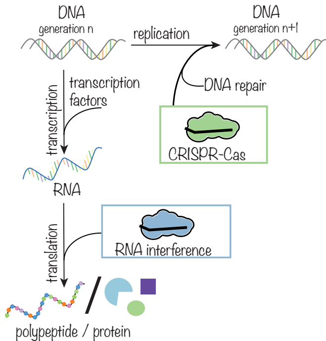
Figure 1.2: The Central Dogma of Molecular Biology states that genetic information is stored as DNA, copied during replication (cell division) and read out by first transcribing it into RNA and then translating it into an amino acid sequence. Each of these processes is heavily regulated by the cell. Target searching proteins play important parts herein: Transcription Factors act on transcription, DNA repair mechanisms safeguard replication. Non-coding RNA guided nucleases fall into this category as well: CRISPR associated (Cas) proteins prevent replication of viral elements, while RNAi controls translation levels.
