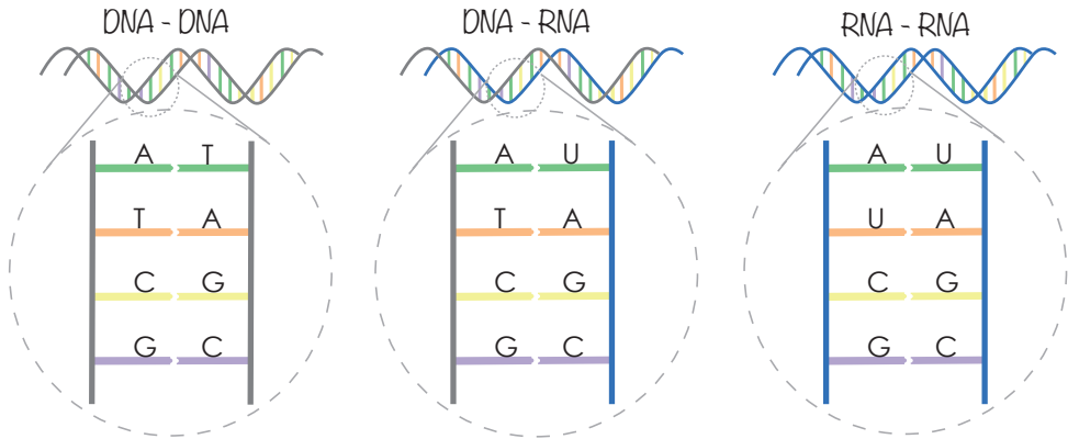
Figure 1.3: Double-stranded nucleic acids form 'base pairs'. (left) DNA-DNA pairs, A(denine) complements T(hymine) and C(ytosine) complements G(uanine). (middle) DNA-RNA pairs, U(racil) replaces T(hymine), thereby matching A(denine). The DNA's Thymine still matches the RNA's Adenine. (right) RNA-RNA pairs, A(denine) complements U(racil). We will refer to any of the shown base pairs as 'matches', while any other possible pair (i.e. A-G) as 'mismatches'.
