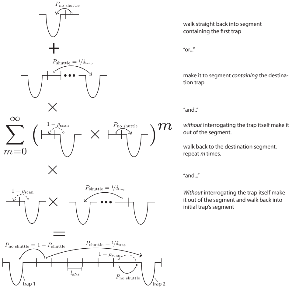
Figure S6.2: related to Figure ??. path counting to derive scaling of shuttling time with distance. A graphical explanation of Equation ???. Subsequent figures will only show the equivalent of the bottom shown here.
