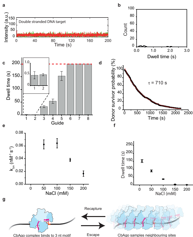
Figure S5.1: Single molecule interactions of CbAgo:siDNA (2-4 nt) at different conditions. (a) Representative trace single-molecule interaction of CbAgo-siDNA (let7) with full target dsDNA target immobilized on the surface (300 per FoV). Exposure time is 100 ms. (b) Dwelltime distribution of CbAgo-guide 3-dsDNA target interactions. Number of molecules recorded n = 540 . Number of datapoints n = 12 (c) Average dwell time of protein bound to target versus guide length for N=1 to N=8 . The error bars are taken from the 95% confidence interval of bootstrapped dwelltimes (20,000 empirical bootstraps). The striped red line indicates the observation time, limited by photobleaching. (d) Survival plot of donor only (Cy3) constructs in standard experimental conditions (100 mM NaCl, 50 mM Tris-HCl pH 8.0). Mean donor bleaching time was obtained by a single exponential fit to the survival probability plot. (e) Binding rate for different salt concentrations for N=3 (nt 2-4) between guide and single target. (f) Dwell time of CbAgo and a single-stranded single target DNA construct ( N=3 ) at 10, 50, 100, 150 and 200 mM NaCl concentration. Total measurement time = 250 s. Error bars are indicating the 95% percentile of 20,000 empirical bootstraps of the mean dwell time. (G) Schematic image indicating the dynamic escape and recapture events of CbAgo.
