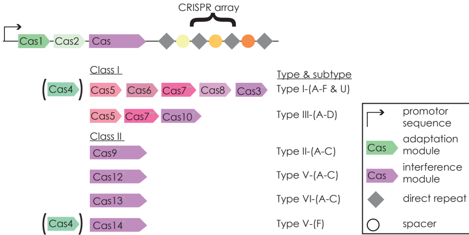
Figure 1.5: Classification of CRISPR systems. Typical architecture of the CRISPR locus is shown on top: The operon controls the adaptation and interference machinery as well as the CRISPR array. Below the most important differences between different types of CRISPR systems in their adaptation/interference modules are shown. For a more elaborate list of CRISPR (sub-)types see [? ]. * signature gene, ** multiple copies present on locus.
