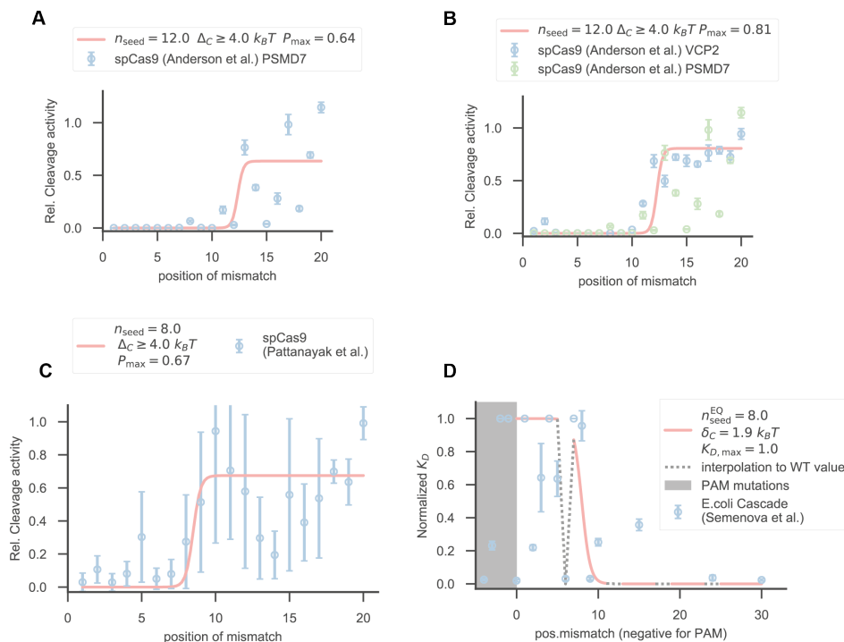
Figure S2.5: Additional comparison to experimental data , related to figure ??
