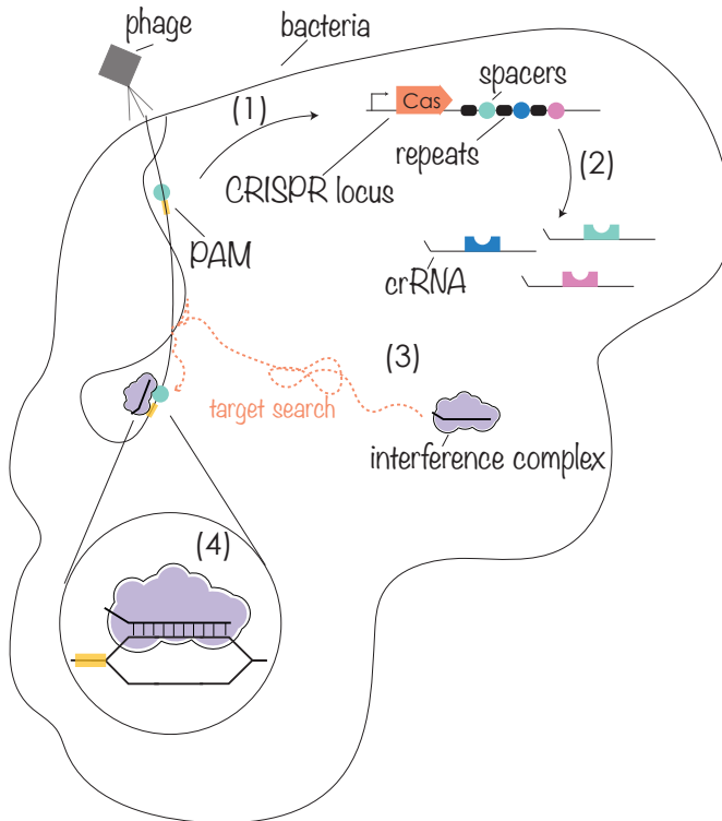
Figure 1.4: The CRISPR-Cas system provides immunity against invading bacteriophages. (1) Upon infection novel spacers are acquired from phage DNA and incorporated in the host' CRISPR locus. (2) Transcription and further biogenesis results in CRISPR-RNA (crRNA) guides. (3) Cas nucleases loaded with the crRNA can search the invading genome for matches to the guide (colored dot) that lie adjacent to a PAM sequence (yellow rectangle). (4) Having found a proper target, the Cas nuclease binds the DNA stably and becomes cleavage competent.
