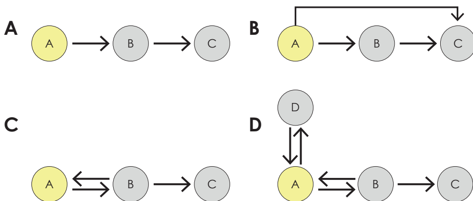
Figure 1.13: Four examples of first passage problems. In each of the figures (A)- (D) we seek the first time we arrive at node C , starting from node A . The probability (density) that this occurs at time t is denoted by \Psi_{AC}(t) .
