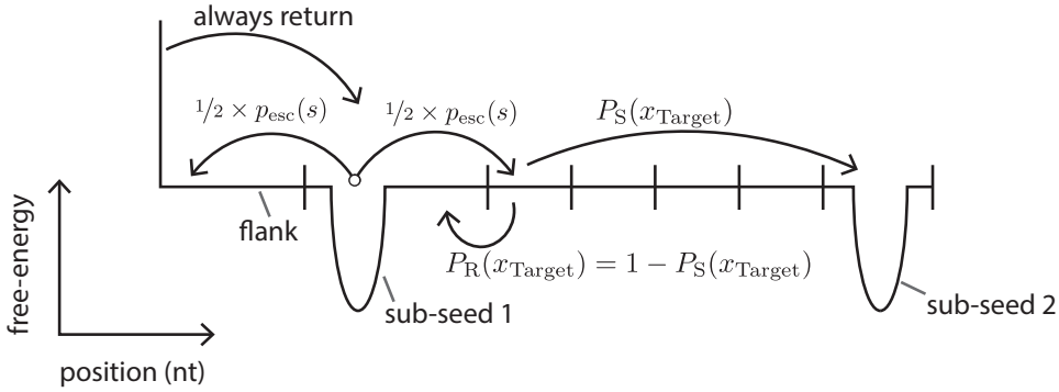
Figure S5.11: This figure illustrates how to construct Equation ?? . Ago slides to either of its neighboring sites with equal probability. Every shuttle event starts with Ago bound to one of the sub-seed sequences. After residing there for a time distributed as p_{esc}(s) , half of the times Ago moves onto the flank (from which it always returns by assumption), while the other half of the times the protein slid onto the poly-T sequence in between the two sub-seeds. All movements along these intermediate sites occur too fast to observe, which is why we only take into account to probability P_S(x_{target}) of completing the shuttle event when x_{target} sites separate Ago from the second sub-seed.
