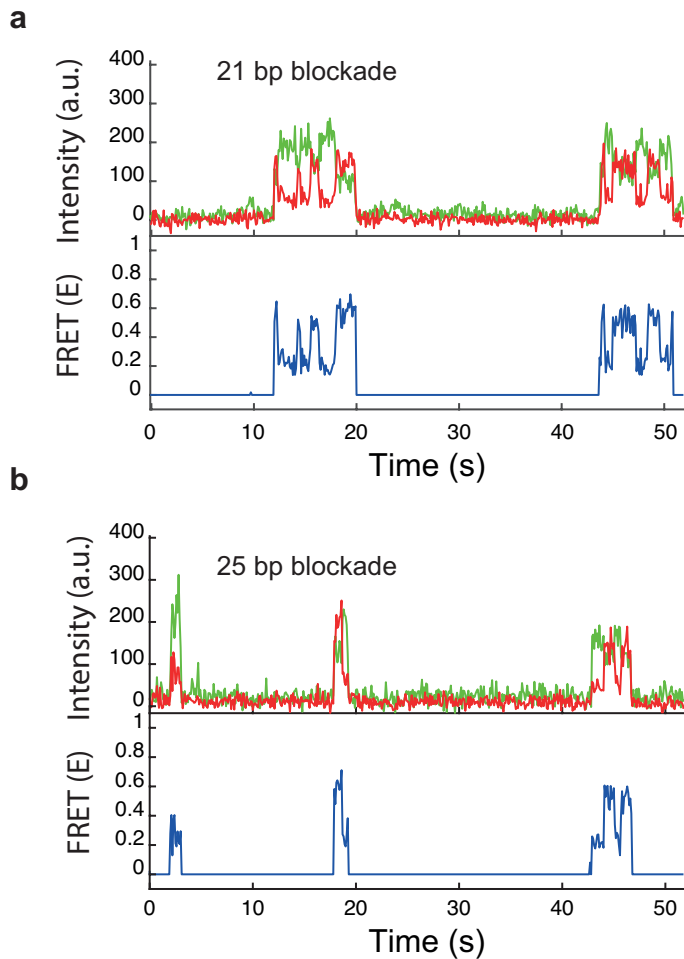
Figure S5.5: Interactions of CbAgo with the dsDNA block construct. (a) Representative trace of CbAgo interacting with a 21 bp DNA blockade construct. (b) Representative trace of CbAgo interacting with a 25 bp DNA blockade construct.
