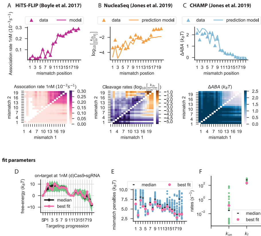
Figure S3.1: related to Figure ??. Fit only to dCas9 data from HiTS-FLIP (Boyle et al.) (A) Comparison of model to HiTS-FLIP data. top: fit against off-targets with 1 mismatch. bottom: fit against off-targets with 2 mismatches (data in upper triangle/ model in lower triangle). (B) Comparison of model to NucleaSeq data. top: prediction of off-targets with 1 mismatch. bottom: prediction of off-targets with 2 mismatches (data in upper triangle/ model in lower triangle). (C) Comparison of model to CHAMP data. top: prediction of off-targets with 1 mismatch. bottom: prediction of off-targets with 2 mismatches (data in upper triangle/ model in lower triangle). (D) Free-energy landscape for 1\text{nM} sgCas9-RNA interaction with on-target DNA. Green curves represent fit results from individual runs of our Simulated Annealing optimization algorithm whose resulting values differ less than 5% from the best-solution's outcomes (figure A) (see S.I.). Black shows median to guide the eye. Pink shows best solution, used to produce figures A-C. (E) Mismatch penalties as a function of position along the RNA-DNA hybrid. Blue dots show individual fit results (after selection). Black shows median to guide the eye. Pink shows best solution, used to produce figures A-C. (F) Forward rate parameters. Green dots show individual fit results (after selection). Black shows median to guide the eye. Pink shows best solution, used to produce figures A-C.
