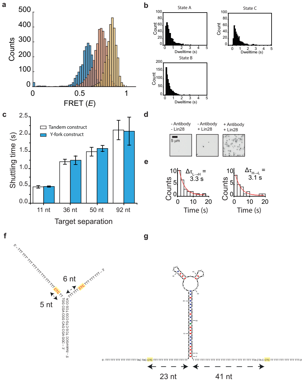
Figure S5.4: Triple target assay, Y-fork assay and Lin28 assay. (a) FRET histogram of three-target assay. n = 168 molecules (b) Dwell time histograms for respectively the low FRET, mid FRET and high FRET state of the three target assay. (c) Shuttling rate of Y-fork constructs (blue) compared to tandem target assay (white) for 11 nt, 36 nt, 50 nt and 92 nt target separation. The error bars indicate the 95% percentile of 20,000 bootstrapped mean dwell times. (d) An EMCCD image of the acceptor channel. (Left) In absence of Lin28 protein and antibody with Cy5 labeled DNA. (Middle) In presence of Lin28 protein and Cy5 labeled DNA. (Right) In presence of antibody, Lin28 protein and Cy5 labeled DNA. (e) Individual dwell times from low FRET state to high FRET state (left) and vice versa (right). (f) Sequence schematic for the Y-fork 11 nt, indicating the target sites and their respective distances to the junction. (g) Sequence schematic for the Lin28 blockade assay, indicating the target sites and their respective distances to the junction/protein.
