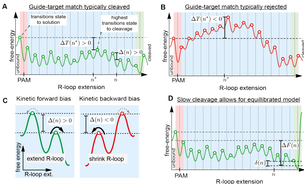
Figure S2.1: General Energy landscapes, related to figure ??. (A) Free-energy landscape underlying the scheme of figure 1A. Our model is completely determined by the set of transition states (open circles). The largest barrier opposing cleavage, is given by the point with the highest drawn transition state (smallest \Delta T ). In the limit of large kinetic biases (see Methods: 'high bias limit' ), it is this barrier that dominates the probability to cleave the target sequence represented. The landscape shown represents a target that is likely cleaved as the largest barrier is opposing unbinding rather than cleavage, or, in other words, the highest transition state lies below the unbinding transition (left most circle). (B) On the contrary, a target will likely get rejected if the highest transition state (placed at n^* ) lies above the transition state towards solution. In this scenario the largest barrier obstructing cleavage is larger than the barrier hindering unbinding. (C) Examples of transitions that bias the RGN to extend the R-loop if the transition state to the right lies below the one to the left (left panel), or to shrink the R-loop if the transition state to the left lies above the one to the right (right panel). The difference in heights of the transition states is referred to as a 'kinetic bias'. (D) Free-Energy landscape as in figure A, in which parameters in equilibrium limit are indicated. Energetic biases ( \delta(n) ) are now set by the stable states within the diagram and their cumulative gain ( \Delta F(n) ) is used to calculate the dissociation constant.
