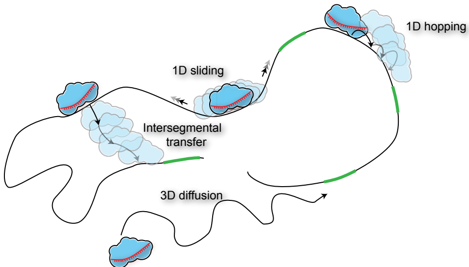
Figure 4.1: Facilitated diffusion. Four different modes of search can in principle be distinguished. 1) 3D search: An Argonaute protein probes a new sequence by first unbinding, then diffusing through the cytosol, and finally binding to probe a new uncorrelated site. 2) Sliding: A non-specifically bound protein laterally diffuses along the mRNA to probe a new site, probing every potential intermediate site from the start to the new site. 3) Hopping: A non-specifically bound protein unbinds, but quickly rebinds again to a site close by (along the RNA) from where it unbound, but not necessarily probing every site in between. 4) Intersegmental transfer: a hopping mechanism where unbinding and binding positions are correlated in 3D space, but far apart along the RNA. This is possible due to the coiled conformation RNA adapts in vivo . binding
