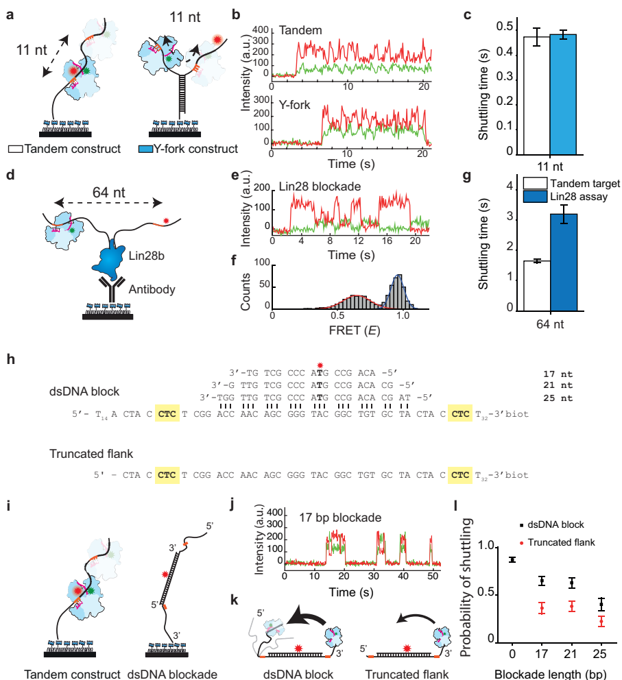
Figure 5.5: Argonaute can overcome structural and protein barriers. a, Schematic drawing tandem target assay (left) and the Y-fork assay (right) with 11 nt separation between targets. b, Representative shuttling traces of the tandem target assay (top) and Y-fork assay. c, The shuttling time of the Y-fork junction (blue bar) compared with the tandem assay (white bar). The experimental data of both sets were taken on the same days. Error bars indicate the 95% confidence interval acquired from 105 bootstraps d, Schematic drawing of the His-Lin28b blockade assay, where targets are separated by 64 nt. Immobilization happens through a biotin-anti-His antibody. e, Example of a shuttling trace with Lin28b located in between two targets. Exposure time is 100 ms. f, FRET histogram (molecules n = 46 ) fit with two Gaussian functions ( E=0.64 for red fit and E=0.95 for dark blue fit). g, The shuttling time of the Lin28 assay compared with the tandem target assay for 64 nt separation between targets. h, Sequences used for the dsDNA block assay, indicating the base pairing between a 17 nt, 21 nt and a 25 nt long blockade and the target strand. The dsDNA block construct has a 19 nt flank on the 5' side, whereas the "truncated flank" has a 4 nt flank. i, Schematic of a dsDNA block assay, where the CTC targets are highlighted with orange. j, Representative trace of binding and shuttling of CbAgo on a 17 bp blockade DNA construct. k, (left) Schematic of dsDNA block construct with full length flanks. (right) schematic of the truncated version where the flank on the 5' side is removed. The thickness of the arrows indicate the observed shuttling probability. l, The probability of shuttling upon binding to a CTC target plotted versus the blockade length (none, 17 nt, 21 nt and 25 nt) for full length flanks (black squares) and for the truncated flanks (red circles). Error bars are given by the 95% confidence interval acquired from 10^5 bootstraps
