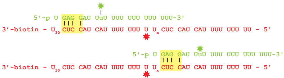
Figure S6.1: related to Figure ??. construct design hAgo2. ssRNA constructs (red) are passivated to the microscope slide using a 3'-biotin-streptavidin linkage. The two trapping sequences, 4 nt sequences that are complementary to the corresponding guide nucleotides (green), are highlighted in yellow. Top figure represents the 'high FRET' configuration, while the bottom figure displays Ago bound to the trap resulting in 'low FRET'. The distance between traps is varied by adding Uracil nucleotides (U x reads: 'x times a U'). To embed the traps within the sequence, as opposed to them being the outermost sites, poly-U sequences flank both traps.
