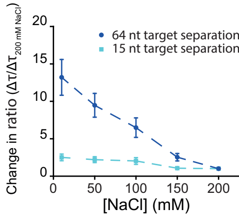
Figure 5.6: The relative change in shuttling time of two constructs from Figure ?? , 64 nt separation (dark blue circles) and 15 nt separation (light blue squares), normalized against \Delta\tau_{shuttle} at 200 mM NaCl. Errors of the ratio were determined through bootstrapping 10^5 times the ratio of \Delta\tau/\Delta\tau_{200\text{ mM NaCl}}
