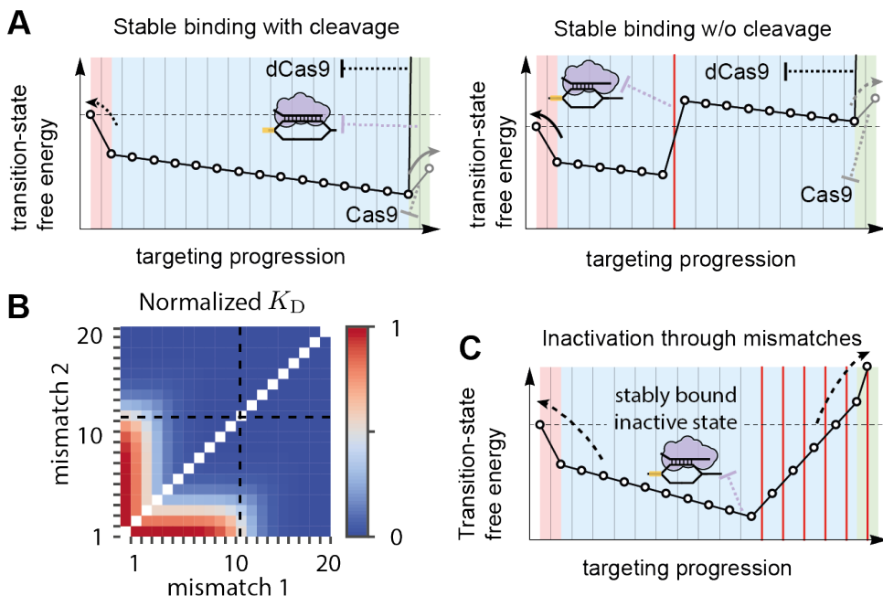
Figure 2.4: Rule (iii) - Differential binding versus differential cleavage. (A) Transition landscapes illustrating the difference between active Cas9 (grey curves) and dCas9 (black curves) when encountering either the cognate site (left panel) or an off-target with a mismatch within the seed (right panel). (B) The dissociation constant for targets with any combination of two mismatches for energetic biases \delta_{\text{PAM}} = 7.5k_B T , \delta_C = 1k_B T and \delta_l = 8k_B T . The end of the seed region is indicated with dashed lines. See figure ?? for single-mismatched off-targets. (C) Transition landscape for an active Cas9 bound to an off-target possessing a block of mismatches placed at the PAM distal end. Even though cleavage is unlikely, unbinding takes a long time.
