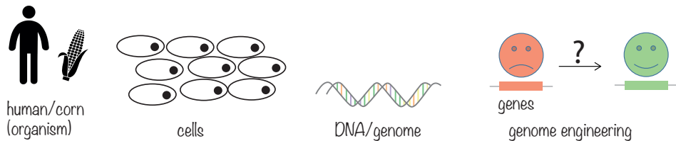
Figure 1.1: Living organisms inherit traits encoded in their DNA. Making (precise) changes to an organisms genome is called 'genome engineering'.
