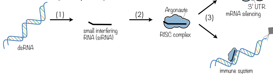
Figure 1.6: RNA interference pathways (in eukaryotes). (A) microRNA pathway:(1) non coding RNA encoded on the genome. (2) 'cropping' by Drosha. (3) Exporting by Exportin 5 and 'dicing' by Dicer. (4) Loading of the guide into Argonaute. (5) RISC complex silences messenger RNA by binding to the 3'-UTR. (B) siRNA pathway:(1) dsRNA in cytosol is processed by Dicer into siRNA.(2) Loading of siRNA into Argonaute. (3) RISC can either silence mRNA or fight-off invading (RNA) viruses.
