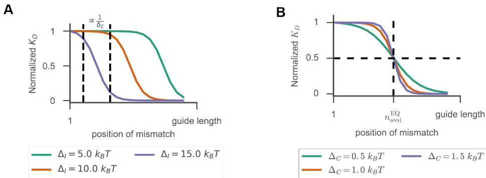
Figure S2.4: Dissociation constant for single-mismatch targets, related to figure ??. (A) Dissociation constant for singly mismatched targets. Fixing \delta_C fixes the width of the curve, the steepness of the transition from seed to non-seed ( \delta_{PAM} = 3k_B T , \delta_C = 1k_B T ). (B) Fixing the ratio between match and mismatch energies fixes the seed length ( n_{seed}^{EQ} through equation ??) ( \delta_{PAM} = 3k_B T , \delta_I = 10\delta_C ).
