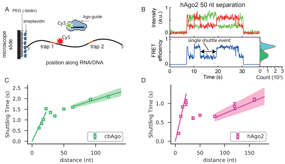
Figure 6.1: Single-molecule FRET experiment to probe lateral diffusion. (A) Schematic of assay. DNA/RNA constructs, containing the two trapping sequences (shown in red) are passivated to the microscope slide via a 3' biotin-streptavidin linker and are labelled with the acceptor dye. The Ago-guide complex is labelled with the donor dye. (B) Representative trace for hAgo2 at a trap separation of 50 nt. Top shows donor (green) and acceptor (red) signals. Bottom shows corresponding FRET efficiency and side panel shows histogram of all FRET efficiency values obtained for the population of molecules. (C) Shuttling time versus trapping distance (average \pm sem) for CbAgo. Solid lines represent linear fits to data points at 11 nt, 15 nt, 18 nt, 22 nt (initial slope) and 64 nt, 92 nt, 120 nt (final slope). Shaded regions represent 95% confidence interval obtained using bootstrapping (see Methods). (D) Same as C for hAgo2. Data points at 7 nt, 11 nt, 15 nt (initial slope) and 80 nt, 120 nt, 160 nt (final slope) are used for linear fits.
