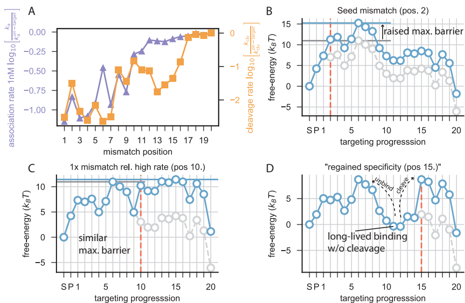
Figure 3.4: Difference between binding and cleavage activities. (A) Association rates from HiTS-FLIP (purple triangles) and cleavage rates from NucleaSeq (orange squares), for single-mismatch off-targets, both normalized to the corresponding on-target rates. (B) Free-energy landscape for off-target (mismatch at position 2) (blue) together with on-target (grey). A seed mismatch significantly raises the largest barrier (horizontal lines) opposing both binding and cleavage. (C) With a mismatch at position 10, binding and cleavage still are limited by the same barrier (horizontal line). Compared to placing a mismatch in the seed (figure B), the off-target landscape (blue) is raised far less in comparison to the on-target landscape (grey). (D) mismatch at position 15 causes binding and cleavage to be limited by different barriers. Binding is stabilized after surpassing the first barrier (entering position 12), whereas cleavage requires Cas9 to surpass also the second barrier visible.
