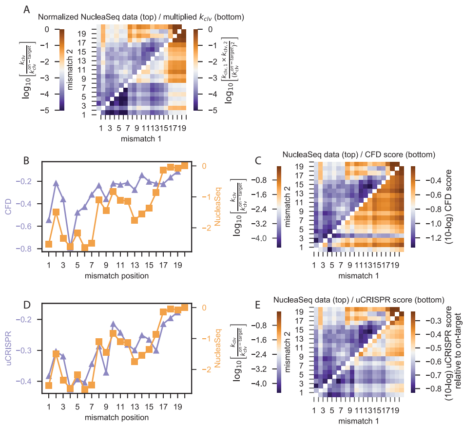
Figure 3.5: Comparison to thermodynamics based models. (A) Upper half shows NucleaSeq data for double mismatched off-targets, normalized to the on-target's rate. Bottom half uses single-mismatch data from Figure ??A as a naïve Bayes classifier to predict the double-mismatch data. For every set of two mismatch positions, the lower half shows the product of the corresponding data points from Figure ??A. (B) Sequenced averaged CFD score compared to NucleaSeq data for off-targets with one mismatch (Figure ??A). (C) Sequenced averaged CFD score compared to NucleaSeq data for off-targets with two-mismatches (upper half Figure ??B) (D) Sequenced averaged uCRISPR score (normalized to on-target) compared to NucleaSeq data for off-targets with one mismatch. (E) Sequenced averaged uCRISPR score (normalized to on-target) compared to NucleaSeq data for off-targets with two-mismatches.
