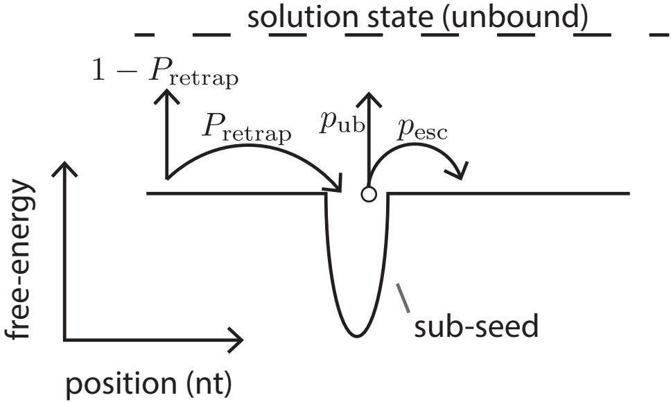
Figure S5.10: This figure illustrates how to construct Equation ?? . Starting from the sub-seed, Ago can either unbind directly (probability p_{ub} ) or slide onto the non-specific binding sites flanking the trap (probability p_{esc} ). When non-specifically bound, Ago can either laterally diffuse back into the sub-seed (probability P_{retrap} ), or unbind (probability 1 - P_{retrap} )
