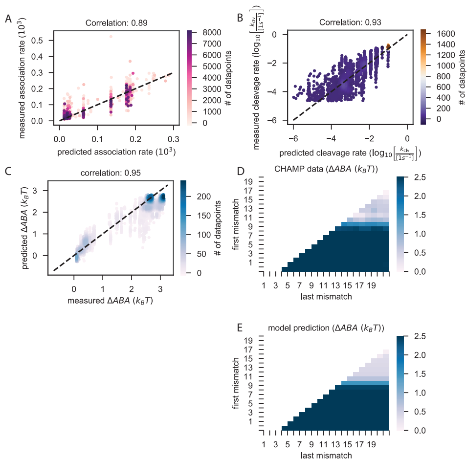
Figure S3.3: related to Figure ??. Correlation plots and additional test data. (A) Correlation of model values (fit+prediction) to HiTS-FLIP data. After making a 2D histogram of the data points, each is assigned a color according to the histogram's bin wherein they lie. Darker color indicates a higher density of data points. Dashed line indicates perfect correlation. Both data fitted against (up until 2 mismatches) and the remainder of the library (>2 mismatches) are included. The latter therefore serves as a test. (B) Correlation of model values (fit) to NucleaSeq data. Orange/Purple indicates a higher/lower density of data points. (C) Correlation of model values (prediction) to CHAMP data. Darker color indicates a higher density of data points. (D) CHAMP data for off-targets with consecutive mismatches. Values on the vertical/horizontal axis indicate the first/final mismatch in the stretch. (E) Model prediction of the data shown in figure D.
