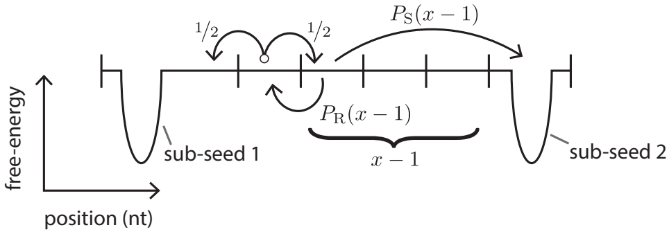
Figure S5.12: This figure illustrates how to construct Equations ?? and ??. Let P_S(x) denote the probability to complete the shuttle when x sites separate Ago from the second sub-seed. Ago walks to either of its neighboring sites with equal probability. Therefore, when situated next to the first sub-seed, Ago gets recaptured half of the times it makes a move, while the other half has a probability of P_S(x - 1) to result in a completed shuttle event.
