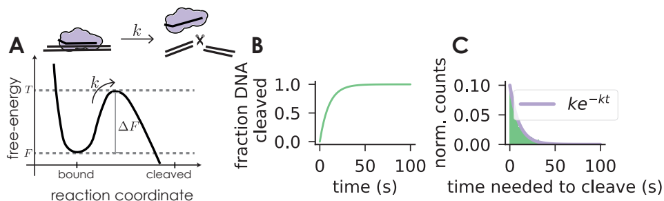
Figure 1.10: A single chemical reaction in which the RGN cleaves its substrate at rate k . (A) Free-energy landscape. A barrier of height \Delta F - the distance from the bound state's free-energy ( F ) to the least favourable intermediate (the transition state T ) - separates the bound from cleaved configurations. (B) Population of cleaved DNA as a function of time. (C) Reaction time for individual reactions - histogram produced generating many realisations - are exponentially distributed.
