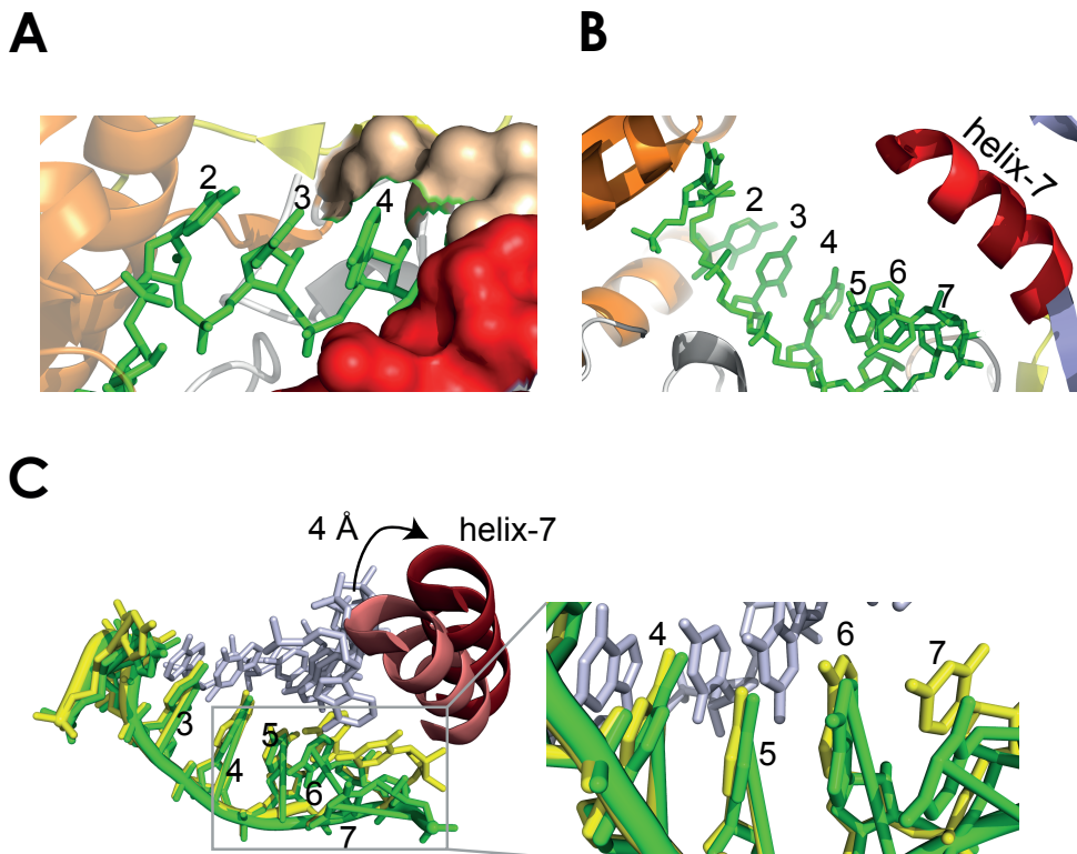
Figure 4.4: Seed of miRNA and hAgo2-helix7. (A) Nucleotides 2–4 (green) of the guide RNA are well exposed by residues in the PIWI domain (golden surface) possibly for initial target recognition (snapshot of the structure 4W5N taken in pymol). (B) (B) The access to nt 5–7 of the guide (green) is blocked by the helix-7 motif (red). The base pairing of target to guide nt 5–7 would require displacement of helix-7 (snapshot of the structure 4W5N taken in pymol). (C) Upon base pairing with the target (grey) the helix-7 motif is displaced by 4 Å compared to guide-only structure. The displacement of helix-7 removes the constraints from nt 6 and 7 (yellow) compared to guide only structure (green) making nt 6 and 7 available for base pairing (see the close-up view in the right panel). (snapshot of the structures 4W5N (guide only) and 4W5O (guide and target) taken in pymol).
