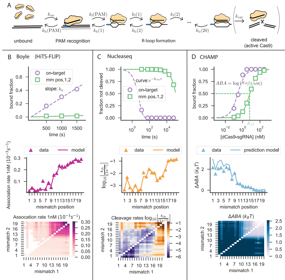
Figure 3.1: kinetic model captures both binding and cleavage data. (A) General reaction schema underlying our kinetic model. A Cas9-sgRNA from the soluble pool (with known concentration) binds the DNA at the PAM site, sequentially progresses through R-loop formation, and eventually cuts the DNA. The set of forward and backward rates describing transitions (arrows) between states (images) fully parameterize our model. (B) Fit to HiTS-FLIP data [? ]. top: the association rate ( k_a ) is estimated as the slope of a straight line forced through the origin and fitted to three measurement points (see S.I.). Figure here shows representative calculations using the extracted model parameters. middle: fit against off-targets with 1 mismatch. Bottom: fit against off-targets with 2 mismatches (data in upper triangle/ model in lower triangle). (C) Fit to NucleaSeq data [? ]. top: the cleavage rate ( k_{clv} ) is estimated by an exponential fit to the fraction of uncut off-target DNA (see S.I.). middle: fit against off-targets with 1 mismatch. Bottom: fit against off-targets with 2 mismatches (data in upper triangle/ model in lower triangle). (D) Prediction of CHAMP data [? ]. top: ABA values are the logarithm of the half-saturation concentration after 10 minutes of dCas9-sgRNA interactions with DNA (see S.I.). middle: prediction of off-targets with 1 mismatch. Bottom: prediction of off-targets with 2 mismatches (data in upper triangle/ model in lower triangle).
