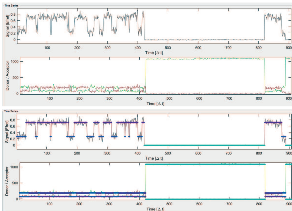
Figure S5.3: Example of HMM software applied to data trace. (Top) An example shuttling trace of CbAgo in the user interface of ebFRET. The donor and acceptor intensities plotted versus time. The donor intensity is enhanced artificially in absence of any signal, resulting in an extra zero FRET state (upper subfigure). (Bottom) The donor, acceptor and FRET intensities overlaid with states resulting from the Hidden Markov Modeling. The HMM analysis program recognizes the unbound state as an extra state (light blue), while low FRET and high FRET are respectively assigned dark blue and purple.
