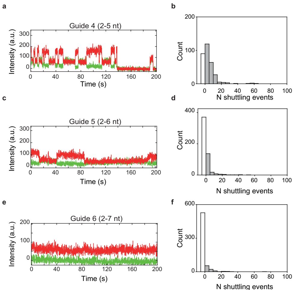
Figure S5.2: Single-molecule interactions of CbAgo with guide 4, 5, 6 and tandem target (22 nt separation). (a) Representative trace of binding events by CbAgo with guide 4 (nt 2-5). Duration of observation 200 s. (b) Shuttling event distribution for guide 4 (nt 2-5). Bin size = 5. The white bar represents binding (no shuttling) events followed by dissociation. N = 317 . (c) Representative trace of binding events by CbAgo with guide 5 (2-6). (d) Shuttling event distribution for guide 5 (2-6 nt). Bin size = 10. The white bar represents events that consists of single molecule binding followed by dissociation. n = 550 . (e) Representative trace of guide 6 (2-7 nt) interaction. (f) Shuttling event distribution for guide 6. The white bar represents events that consists of single molecule binding followed by dissociation. n = 621 .
