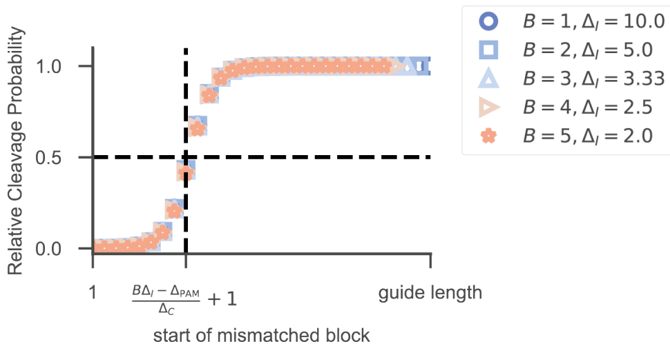
Figure S2.3: Block of mismatches, related to figure ??. The probability to cleave a target with B consecutive mismatches is equal to the probability to cleave a target with a single mismatch (placed at the start of the block) and with a mismatch bias scaled by the length of the block ( \Delta_C = 1k_B T , \Delta_{PAM} = 2k_B T , \Delta_{clv} = -100k_B T ).
