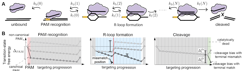
Figure 2.1: Kinetic model of RGN target recognition. (A) The RGN initially binds its substrate at the PAM site, from which it can either unbind with rate k_b(0) , or initiate R-loop formation with rate k_f(0) . A partially formed R-loop of length n grows to length n + 1 with rate k_f(n) , or shrinks to length n - 1 with rate k_b(n) . Eventually, the RGN will either cleave its substrate with rate k_f(N) or reject the substrate and unbind with rate k_b(N) . In the special case of a RGN that does not utilize PAM binding, it is assumed to bind straight into the initial state of R-loop formation. (B) The transition landscape of our minimal model. In the left panel, we illustrate a PAM bound enzyme kinetically biased toward R-loop formation by different amounts (black, grey, and light grey curves). The kinetic bias for the canonical PAM shown as \Delta_{PAM} . In the middle panel we illustrate two kinetic biases toward R-loop extension (black and grey curves), with the larger bias indicated as \Delta_C . In the same panel we further illustrate two kinetic biases against R-loop extension (grey and light grey curves) at mismatches (red vertical lines), with the largest bias shown as \Delta_I . Once the complete R-loop is formed, the system is kinetically biased against cleavage by \Delta_{C/I}^{clv} = \Delta_{C/I} \mp \Delta_{clv} , as dictated by the nature of the terminal base pairing. See Figure ?? for complete energy landscapes.
