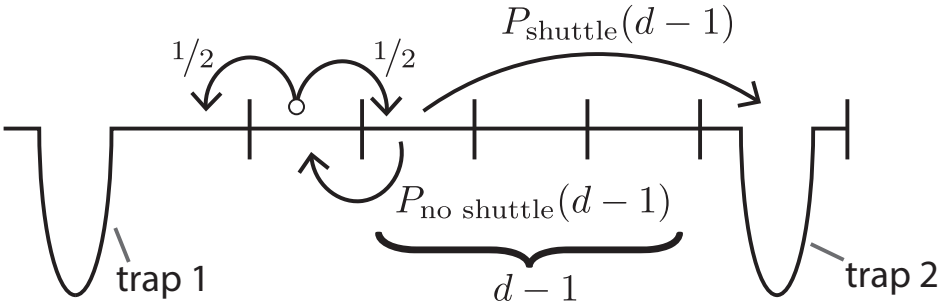
Figure S6.3: related to Figure ?? . Shuttling time simple diffusion scales linearly with d_{\text{trap}} . Illustration of recursion relation dictating probability to shuttle P_{\text{shuttle}} (or get recaptured P_{\text{no shuttle}} ) in terms of number of binding sites separating the two traps. Relates to Equations ?? and ??.
