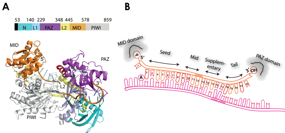
Figure 4.3: Structural and domain overview of hAgo2 and miRNA. (A) The binary structure of hAgo2-miRNA showing four well conserved domains among Argonaute proteins (snapshot of the structure 4W5N taken in pymol) (B) Argonaute proteins divide miRNA (orange) into several domains. The 5' phosphate and nt 1 of miRNA (anchor) is bound to the pocket in the MID domain. The nt 2–8 are known as seed sequence, as they are crucial for initial targeting. The nt 9–10 have the least significant role in target recognition and are known as the mid region. The 3' supplementary region is comprised of nt 13–16, they also have considerable role in stabilizing miRNA-target interaction. The nucleotides beyond the 16th do not base pair with the target and are called the tail region. The 3' OH is bound to the binding pocket in PAZ domain making it as a 3' anchor. The t1 Adenosine (t1A) in the target RNA (pink) binds to the binding pocket in MID domain..
