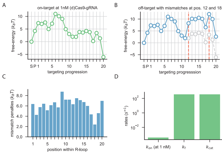
Figure 3.2: Kinetic parameters. (A) Free-energy landscape representing on-target DNA interacting with 1nM Cas9-sgRNA. (B) Free-energy landscape representing off-target DNA (mismatches at positions 12 and 18) interacting with 1nM Cas9-sgRNA (blue). On-target free-energy landscape shown in grey. (C) Mismatch penalties as a function of location within RNA-DNA hybrid. (D) Forward rate parameters.
