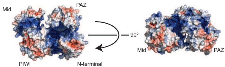
Figure S5.9: Coulombic surface coloring of Clostridium butyricum Argonaute (CbAgo). The crystal structure of CbAgo (PDB 6qzk) (3.23 Å resolution) reveals the charge distribution. The left that contains the guide DNA and the target DNA is highly positively charged (blue).
