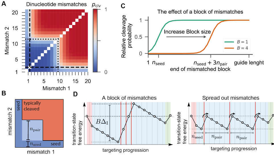
Figure 2.3: Rule (ii) – mismatch spread. (A) The relative-to-wildtype probability to cleave a target with two mismatches for a system with \Delta_{PAM} = 3.5k_B T , \Delta_1 = 4k_B T , \Delta_C = 1k_B T and \Delta_{clv} = 1k_B T . The seed length n_{seed} is indicated with dashed lines, and n_{seed} + n_{pair} is indicated with dotted lines. (B) Schematic of the probability to cleave a target with two mismatches. The target is typically rejected in both blue regions and rejected in the red. (C) Probability to cleave a target with a block of B mismatches as a function of the location of the last mismatch. Also see ???. (D) Spreading out blocked mismatches (left panel) around their average position significantly lessens the barrier to cleavage (right panel).
