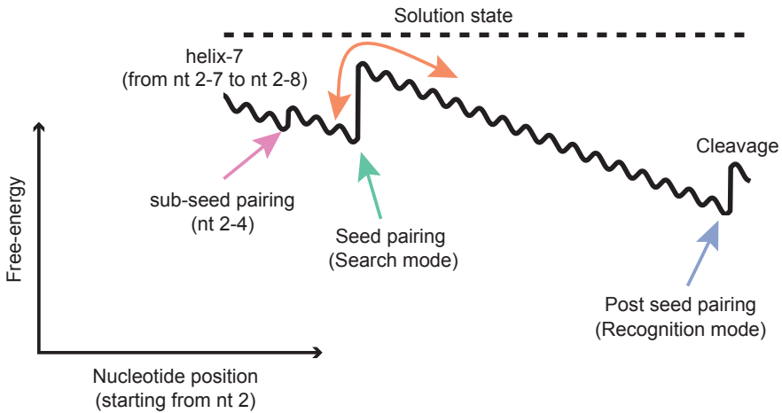
Figure 4.6: Target search process by hAgo2. (A) A model summarizing conformational changes during target search by hAgo2-miRNA. In light of the search-stability paradox discussed in Fig. ?? we identify a two search modes (pink + green) and a recognition mode (blue). Alternating between search and recognition modes is enabled through the movement of the helix-7 motif (orange). (B) Schematic free-energy diagram for Ago-microRNA target recognition. Forming bonds between target and guide (horizontal axis) makes the complex more stable (vertical axis). In light of the search-stability paradox, as proposed by Slutsky and Mirny and discussed in Fig. ??, we identify at least 1 search mode (pre-seed pairing, green arrow) and at least one recognition mode (post-seed pairing, blue arrow). To resolve the paradox, Argonaute can use the movement of its helix-7 motif to switch between search and recognition modes (orange arrow). Potentially, additional modes can be distinguished, such as sub-seed pairing (pink arrow).
