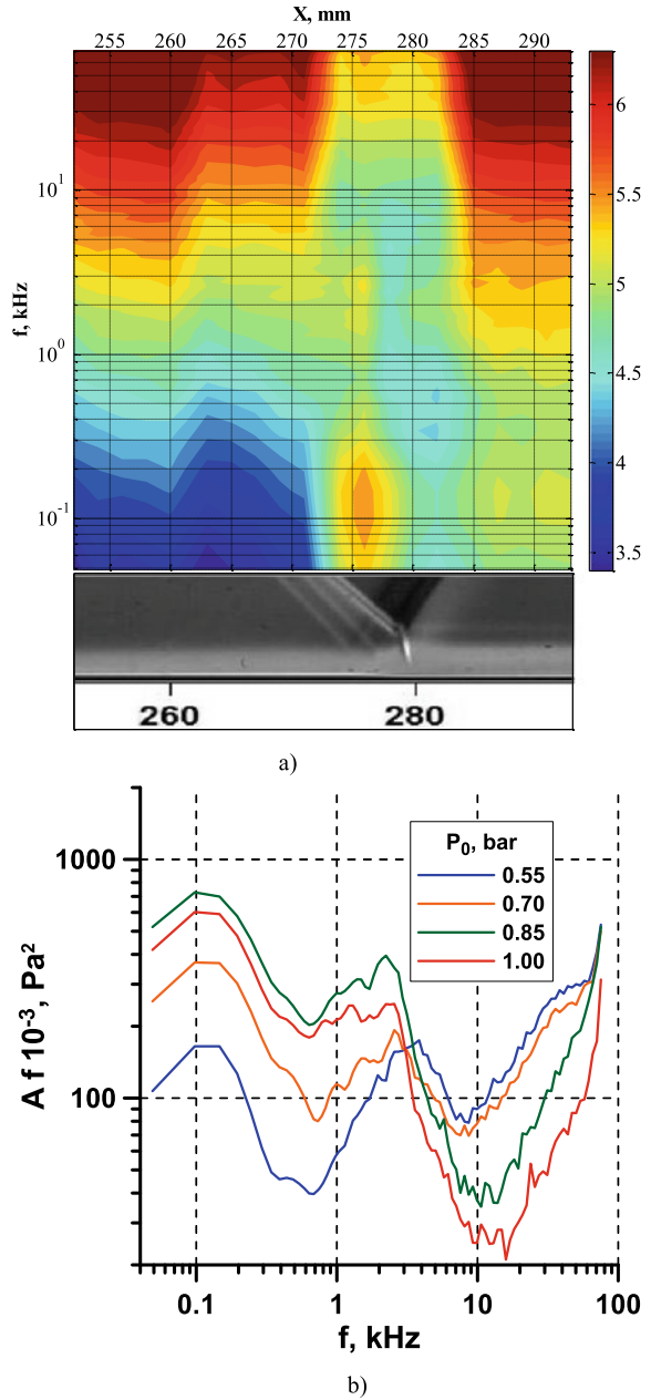
Fig. 64 PSD:f of wall pressure pulsations for turbulent test case a along zone of SWBLI ( L = 100 mm, \beta = 4^\circ , P_0 = 0.7 bar) and b at point of maximum pulsation for various P_0
