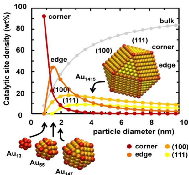
Figure 1.3 Density of adsorption sites ((001), (111), edge, or corner on-top sites are marked with light orange, yellow, dark orange, or red symbols represent, respectively) on closed-shell cuboctahedral Au clusters as a function of the cluster diameter. Gray dots represent the weight fraction of Au bulk atoms. [40]
