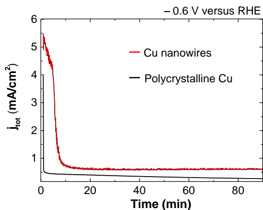
Figure S2.1.8 CO 2 reduction current as a function of time at -0.6 V vs. RHE.
