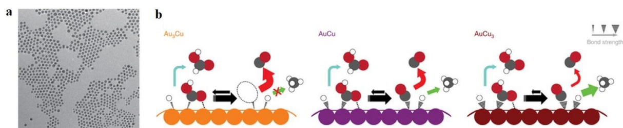
Figure 1.13 (a) TEM image of AuCu 3 NPs (scale bar, 100 nm). (b) Schematic illustration of the proposed mechanism for CO 2 reduction on the Au–Cu bimetallic NPs. Filled circles with grey, red and white color represent C, O and H, respectively. On the top right corner, the relative binding strength of intermediate is marked with the stroke weight. A dotted line indicates the additional binding between the COOH and the catalyst surface. Black horizontal arrows show the difference in probability of having COOH intermediate on different catalysts. The pathway towards each product is indicated by colored arrows (red: CO; blue: HCOOH; green: hydrocarbons). [52]
