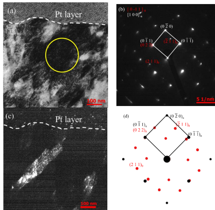
Figure 10. The (a) BF image of another area in the WEL-interface TEM specimen; (b,d) SAD pattern and indexed pattern, respectively, of the region enclosed in the circle shown in (a). The DF image in (c) is obtained from the (211) reflection of cementite.
