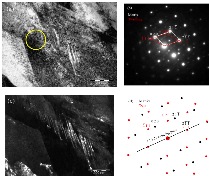
Figure 7. (a) A BF image of the WEL surface in the TEM foil; (b) Selected area diffraction (SAD) pattern, corresponding to zone axis [102]matrix of the region enclosed in the yellow circle; The (c) DF image formed from the (\bar{2}11) reflection of the twinning plane and (d) simulated diffraction pattern corresponding to (b).
