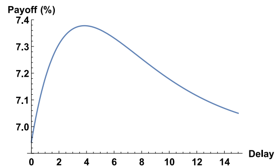
Fig. 3. The patient’s payoffs relative to a healthy individual’s after completing two rounds as a function of round 3’s delay with toxicity rate z_2 = 0.73 and facing a cure rate of \lambda_3 = 0.3 . Expected payoffs are maximized at a delay of \hat{t}_3 = \ln(z_2/\hat{z})/\zeta = 3.86 .
