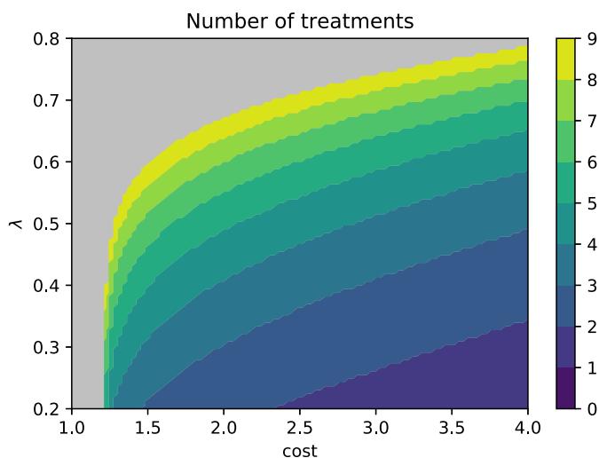
Fig. 2. Optimal number of treatment rounds in the cost-based model for parameter values shown in Table 1. Gray areas show the regions in which more than 9 rounds of therapy is optimal. The progressive disease state at which the patient should cease therapy increases with the likelihood of cure and decreases with the cost to the patient in terms of money, lost income or ill-health from therapy.
