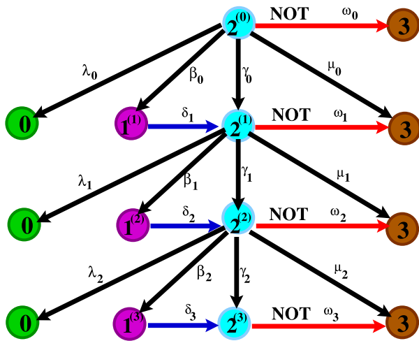
Fig. 1. Schematic showing transition rates of the first 3 decision nodes of therapy. Each 0 node and each 3 node on the figure represent one absorbing state, while the figure shows multiple copies for better visibility. From an undetectable disease state, 1^{(i)} , the patient will eventually progress to detectable state 2^{(i)} . If the patient opts for therapy, he or she progresses to one of the four states 0, 1^{(i+1)} , 2^{(i+1)} , or 3. Otherwise, by choosing the no therapy option, he or she eventually progresses to state 3.
