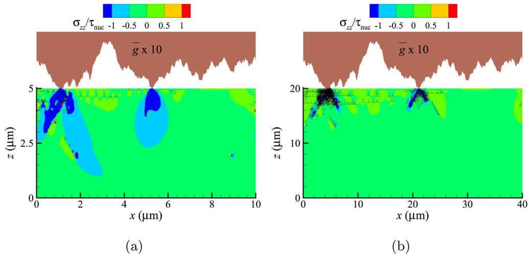
Fig. 7. Stress and dislocation distribution in two crystals with (a) z_m = 5 \mu\text{m} , \bar{h} = 0.05 \mu\text{m} and (b) z_m = 20 \mu\text{m} , \bar{h} = 0.2 \mu\text{m} at strain u_z/z_m = 0.002 . The rms height of the indenter is also scaled with z_m , and magnified by a factor of 10 in z – direction for better visualization.
