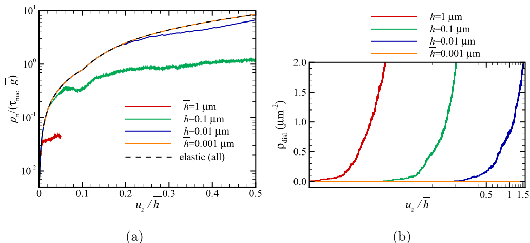
Fig. 8. (a) Normalized nominal contact pressure for different rms heights. All elastic curves overlap. Also, the curve corresponding to the plastic response of the crystal with rms height \bar{h} = 0.001 \mu\text{m} overlaps with the elastic curve, but will deviate at larger indentation depth. (b) Dislocation density \rho_{\text{disl}} in the crystal is plotted for different rms heights.
