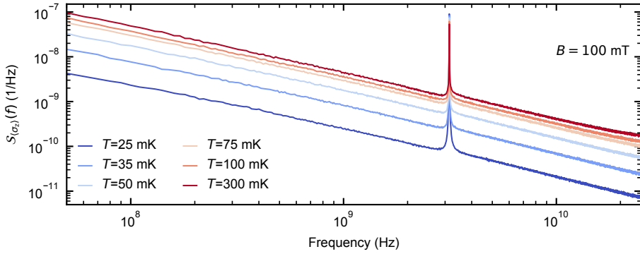
Figure 1.5: Spectrum of the switcher traces, averaged over different switching rates. The field is fixed at 100 mT while the temperature is changed. The 1/f background increases with temperature. Correspondingly, the peak due to the hyperfine interaction reduces in magnitude.
