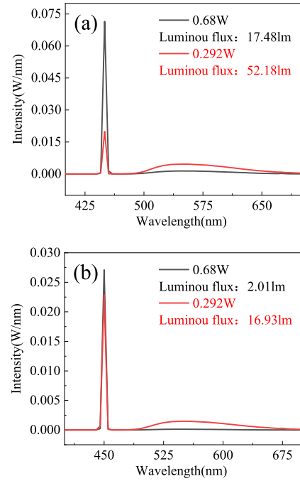
Fig. 5. The SPDs of 10% YAG: Ce^{3+} phosphor/silicone composite measured under (a) R-mode; and (b) T-mode integrating sphere 2.
