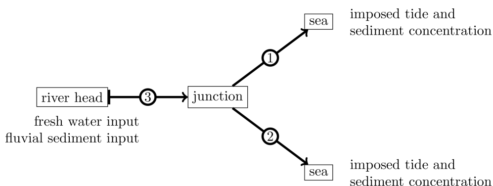
FIGURE 2 Sketch of the three-channel estuarine network considered in this study. Numbers in circles indicate channel numbers.
