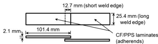
Figure 1. Lap shear specimen geometry. CF/PPS: carbon fiber/polyphenylene sulfide.
