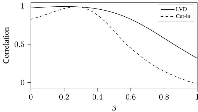
Fig. 11. Correlation between the medians of M_1(\mathcal{W}^*, \mathcal{Z}^*, \lambda^*) (open circles in Figs. 9 and 10) and \tilde{W}_1(\mathcal{Z}_{\text{large}}^*, \mathcal{W}^*) (filled circles in Figs. 9 and 10) for different values of \beta . The solid line shows the result for the LVD scenarios with a maximum correlation of 0.992 at \beta \approx 0.21 . The dashed line shows the result for the cut-in scenarios with a maximum correlation of 0.987 at \beta \approx 0.27 .
