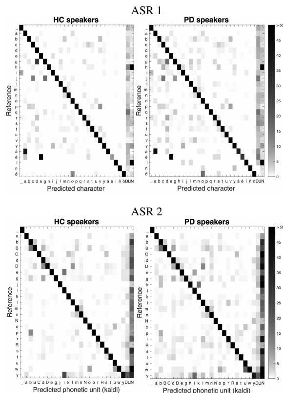
Figure 3: Character substitution, insertion and deletion rates (%) per character in ASR 1 (top) and phonetic unit in ASR 2 (bottom). The two last columns labeled as DL and IN are deletion and insertion error rates, respectively. <-> represents the space character.
