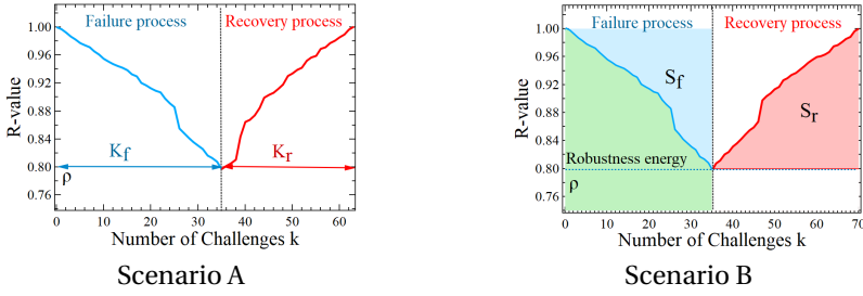
Figure 6.2: Illustration of the failure process and the recovery process in an Erdős-Rényi (ER) random graph G_{0.1}(100) with link density p = 0.1 and network size N = 100 in one realization. The R -threshold is \rho = 0.8 .
