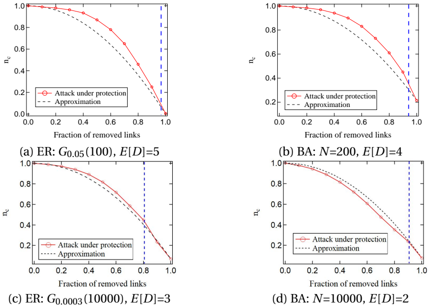
Figure 5.10: The normalized maximum number of controllable nodes n_c as a function of the fraction of removed links l in synthetic networks under random attacks with protection. The results for each fraction l is based on 10000 simulations. In each sub-figure, the vertical dashed line marks the position where l = 1 - l_c .
