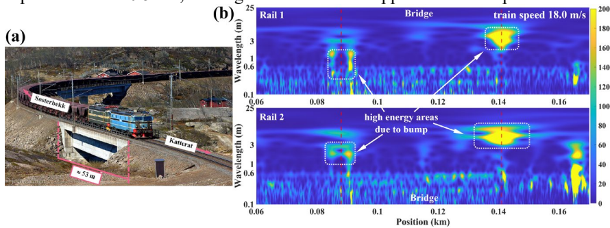
Fig. 5. ABA measurement at a bridge in Norway
