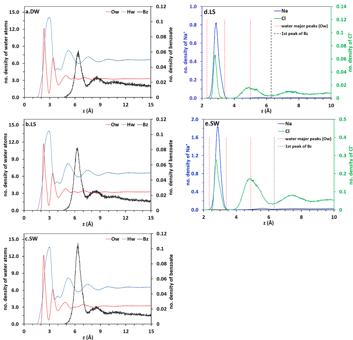
Figure 1. Density profile of (a–c) oxygen and hydrogen atoms of water (Ow/Hw) and benzoates (Bz) and (d, e) \text{Na}^+ – \text{Cl}^- ions in different brines. Maxima of water density (based on Ow) and Bz are outlined in (d) and (e) for the sake of clarification of position of ions. The data was averaged over both calcite slabs but presented for one of the interfaces.
