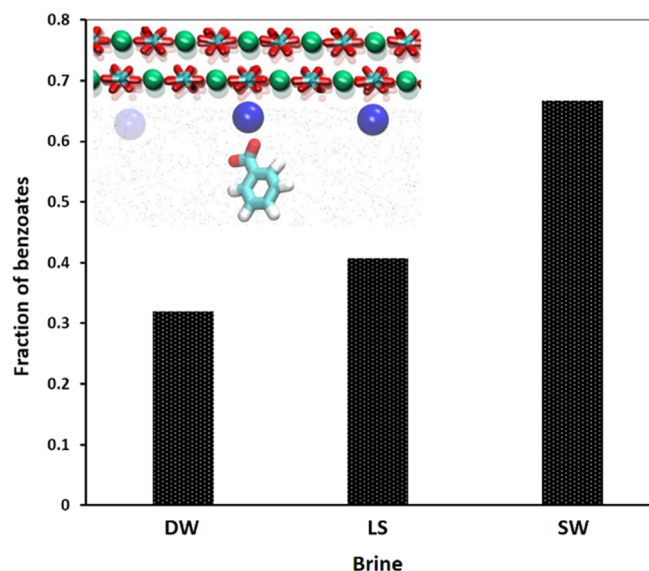
Figure 10. Fraction of benzoates at the interface that pair to \text{Na}^+ ions of the Stern layer. (Inset: Schematic representation of the ability of \text{Na}^+ ions to serve as a potential adsorption site for benzoates onto calcite.)
