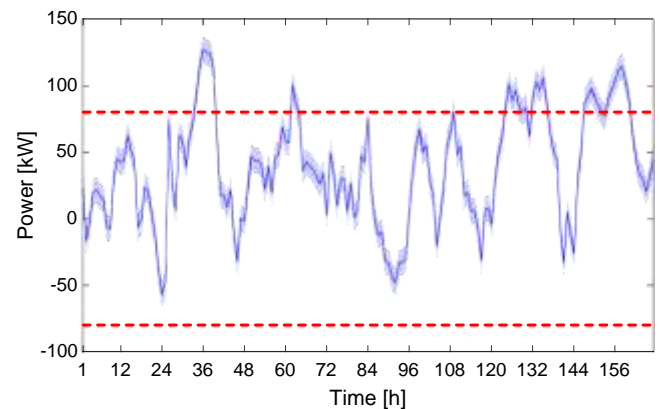
Fig. 2. Residual load of the microgrid; shaded area indicates the uncertainty and the red lines are the limits on the power exchange between the microgrid and the power network.
