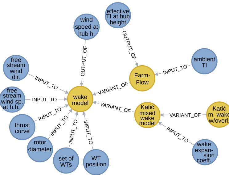
Figure 16. Example of an ordered set of variant models and their variables (excerpt from WESgraph).
