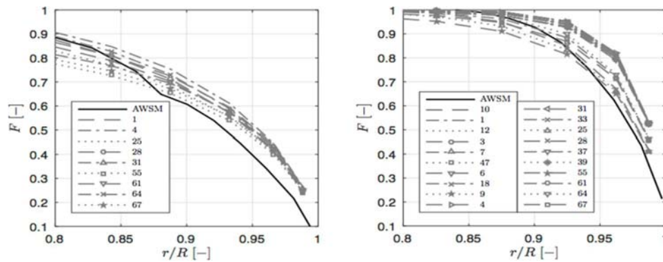
Figure 8: Different implementation of Prandtl tip loss factor as function of radial position compared with tip loss factor from ASWM for a constant loading variant of the Mexico variant. Left: \lambda = 4.9 and right \lambda = 11.9
