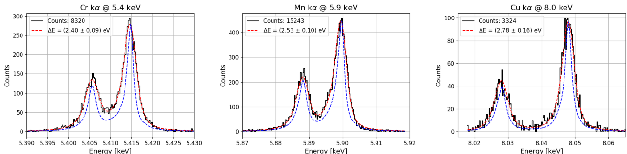
Fig. 5. Best fit to data (red lines) for each detected K\alpha line (MXS and internal 55Fe X-ray source) for Px1 biased at @ 1.1 MHz. The lines intrinsic shape (blue lines) has been described according to [16].
