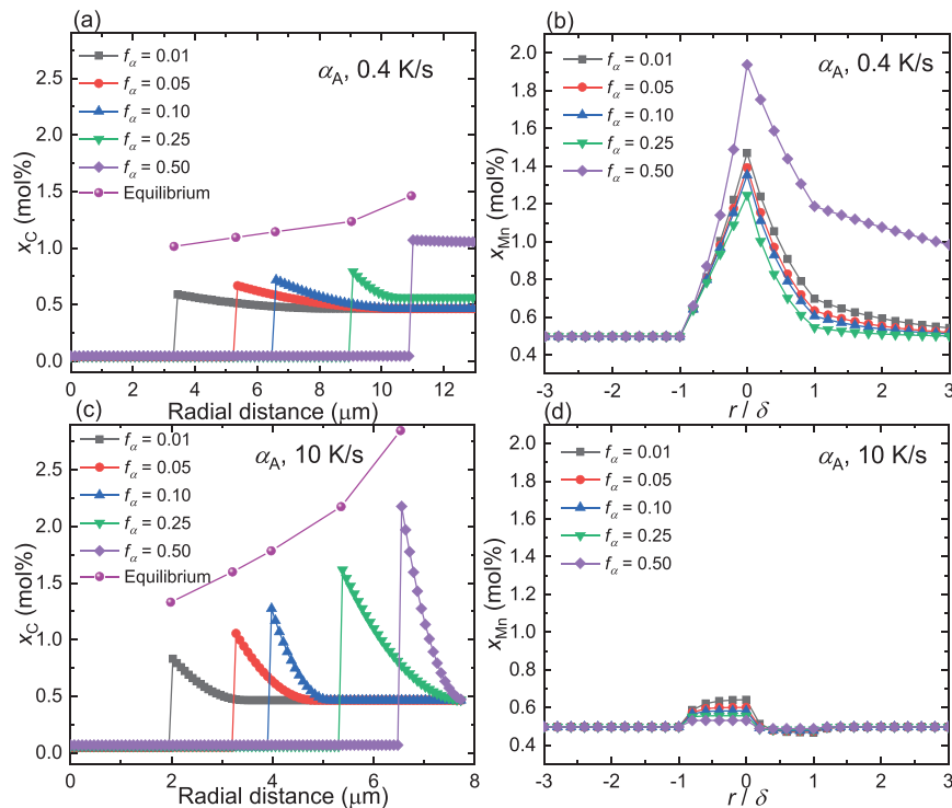
Fig. 4. Carbon (a, c) and manganese (b, d) profiles across the interface for grain \alpha_A (as visualized in Fig. 3) at cooling rates of (a, b) 0.4 K/s and (c, d) 10 K/s. r / \delta is a dimensionless quantity where r is distance and \delta is the half of the interface thickness.
