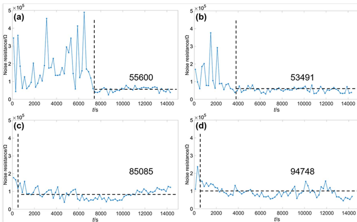
Figure 3. Noise resistance calculated for AA2024-T3 initially exposed in 0.01 M NaCl and 0.01 M \text{Li}_2\text{CO}_3 solution for 14500 s (approximately 4 h) and subsequently exposed in 0.01 M NaCl after ambient ageing for (a) 0 h, (b) 4 h, (c) 24 h, and (d) 72 h. The vertical dashed lines indicate the transition from inhibition to corrosion stage. The numbers (unit: \Omega ) shown in the figure indicate average noise resistance values in the corrosion stage.
