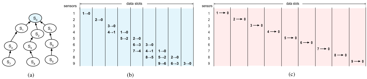
FIGURE 8. Sample 9-flow network with schedules for optimal source routing (HRP) and Blink. The slot length for HRP and Blink is 10 ms and 20 ms, respectively. (a) Topology. (b) HRP, completion in 90 ms. (c) Blink, completion in 180 ms.
