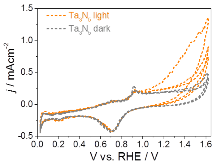
Figure 4.2.3. JV curve of the bare 225 nm \text{Ta}_3\text{N}_5 in the dark and under AM1.5 illumination in 1 M KOH. The scan rate is 50 mV/sec.
