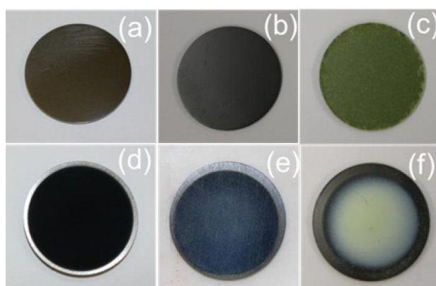
Figure 3.4 Photographs of (a) polished tungsten, (b) polished tungsten after two-step anneal at 550/450°C, (c) polished tungsten after anneal at 700°C, (d) nanostructured tungsten, (e) nanostructured tungsten after two-step anneal at 550/450°C, and (f) nanostructured tungsten after anneal at 700°C.
