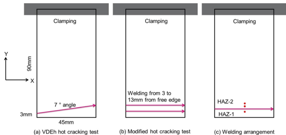
Fig. 1 Schematic top view of a standard self-restraint hot cracking test (VDEh), the red line indicates the weld center line; b modified hot cracking test at increasing distances parallel to the free edge; and c welding arrangement in this study: transient temperature is measured in HAZ-1 at 3 mm from the weld center line and HAZ-2 at 2.5 and 4 mm from the weld center line
